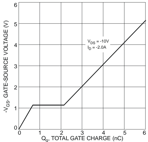
Fig. 10 Gate-Charge Characteristics
