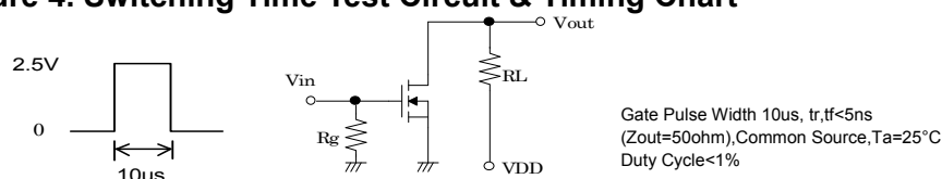
Figure 4. Switching Time Test Circuit & Timing Chart
