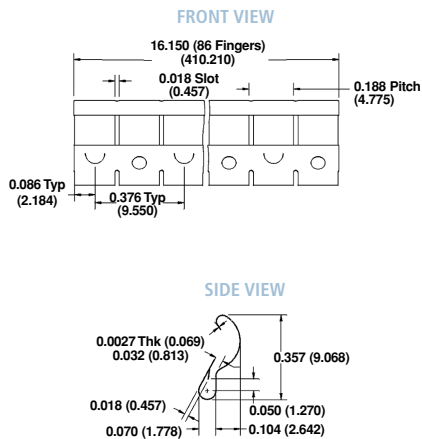
TRANSFER IMPEDANCE TEST PART NO. 97-636
