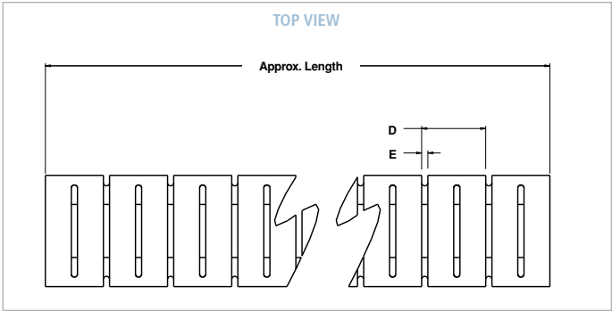
Part No. 77-075, 77-093, 77-110
