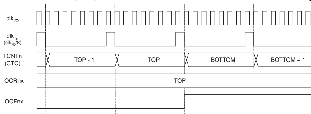
Figure 16-11. Timer/Counter Timing Diagram, Clear Timer on Compare mode, with Prescaler ( f_{clk\_I/O}/8 )
