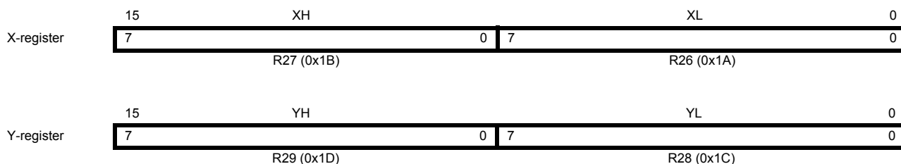
Figure 8-3. The X-, Y-, and Z-registers
