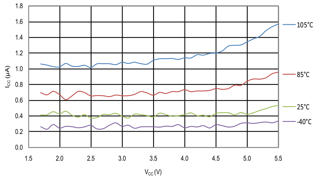
Figure 31-11. ATmega48PB/88PB: Power-Down Supply Current vs. V CC (Watchdog Timer Disabled)
