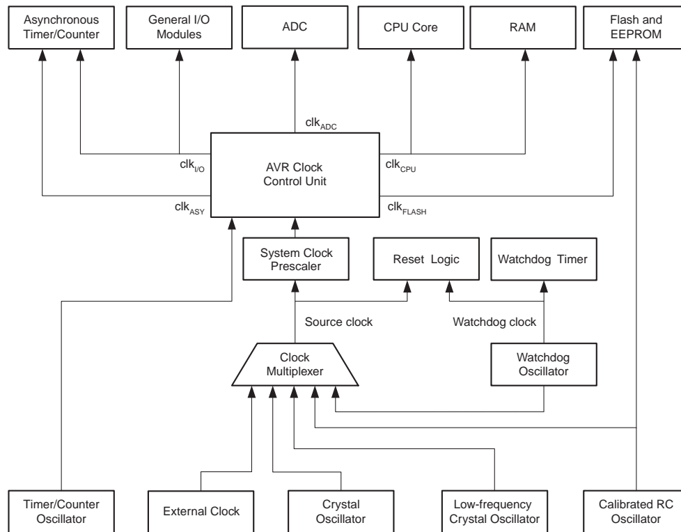
Figure 10-1. Clock Distribution
