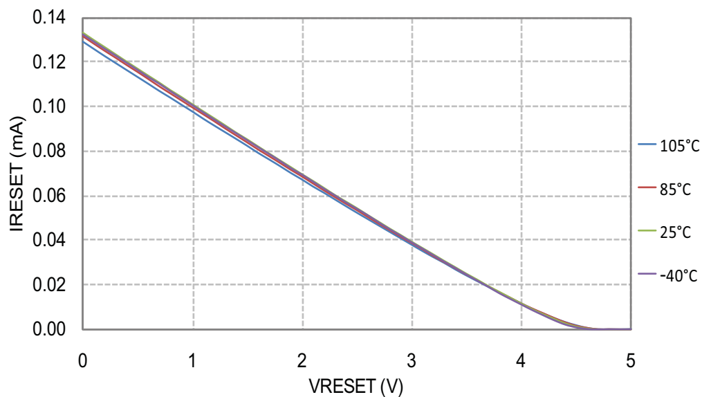
Figure 31-64. ATmega168PB: Reset Pull-up Resistor Current vs. Reset Pin Voltage ( V_{CC} = 5V )
