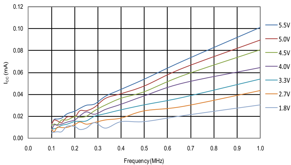
Figure 31-44. ATmega48PB/88PB: Reset Supply Current vs. Low Frequency (0.1MHz - 1.0MHz)
