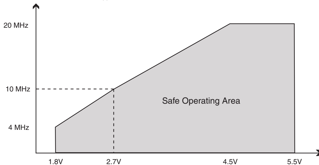
Figure 30-1. Maximum Frequency vs. V_{CC}
