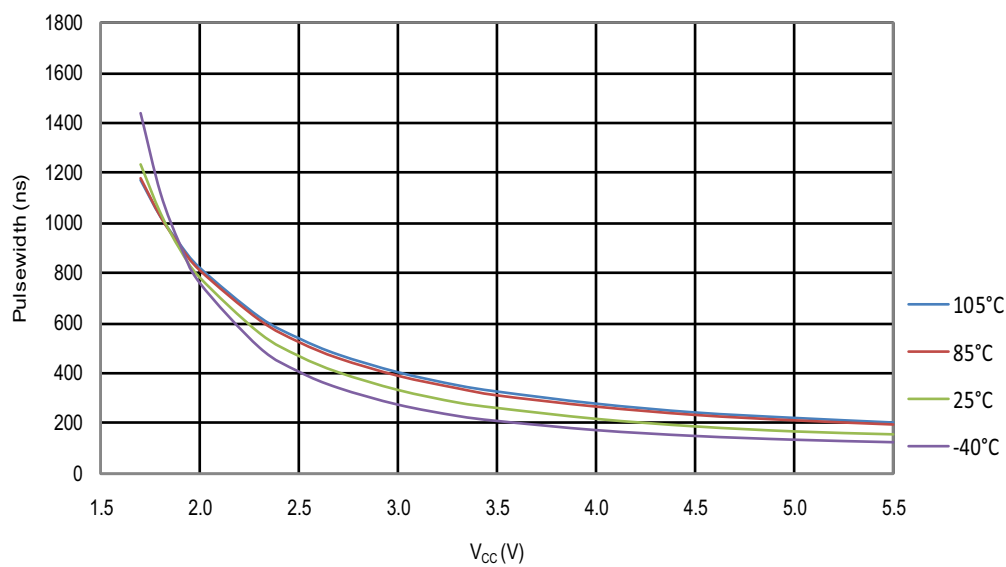
Figure 31-46. ATmega48PB/88PB: Minimum Reset Pulse Width vs. Vcc
