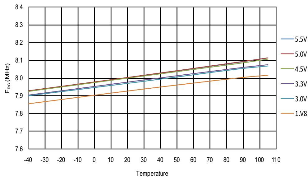
Figure 31-37. ATmega48PB/88PB: Calibrated 8MHz RC Oscillator Frequency vs. Temperature
