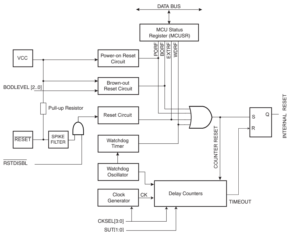
Figure 12-1. Reset Logic
