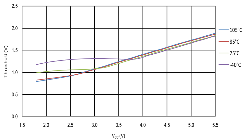
Figure 31-26. ATmega48PB/88PB: Reset Input Threshold Voltage vs. V_{CC} ( V_{IH} , I/O Pin read as '1')
