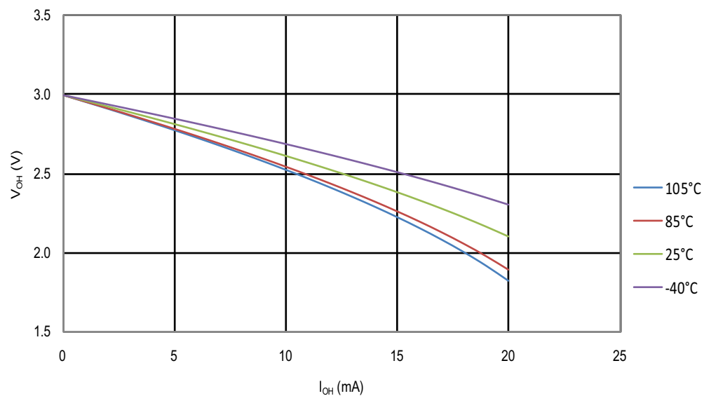
Figure 31-21. ATmega48PB/88PB: I/O Pin Output Voltage vs. Source Current ( V_{CC} = 3V )
