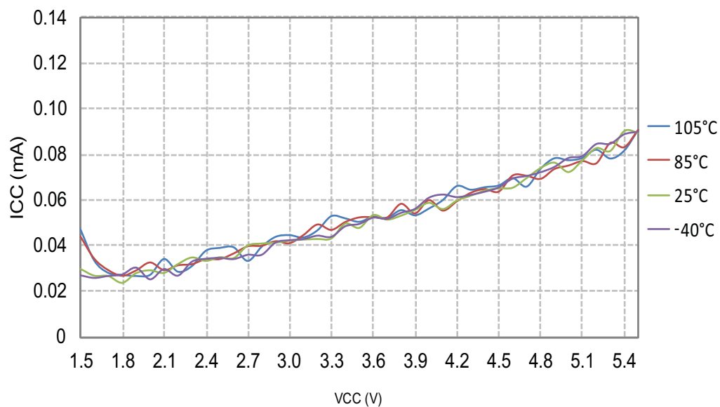
Figure 31-50. ATmega168PB: Active Supply Current vs. V_{CC} (Internal RC Oscillator, 1MHz)
