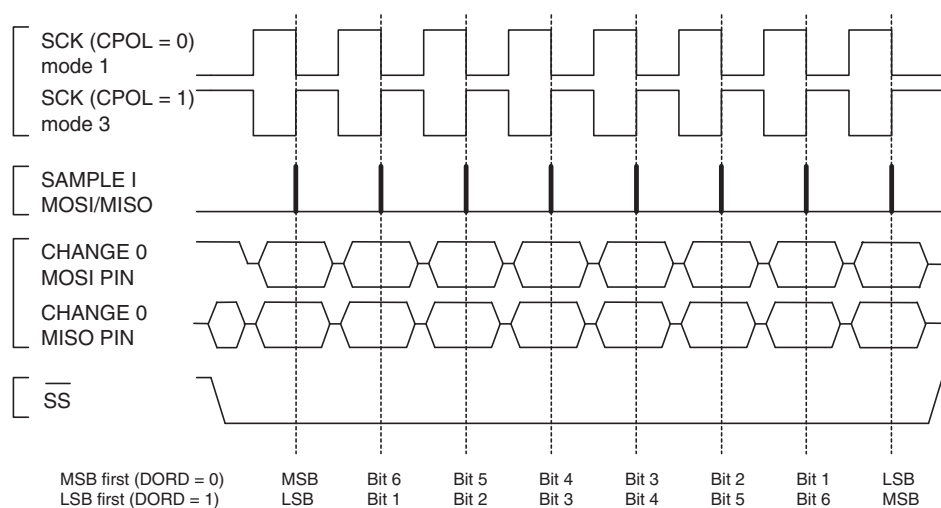
Figure 20-4. SPI Transfer Format with CPHA = 1
