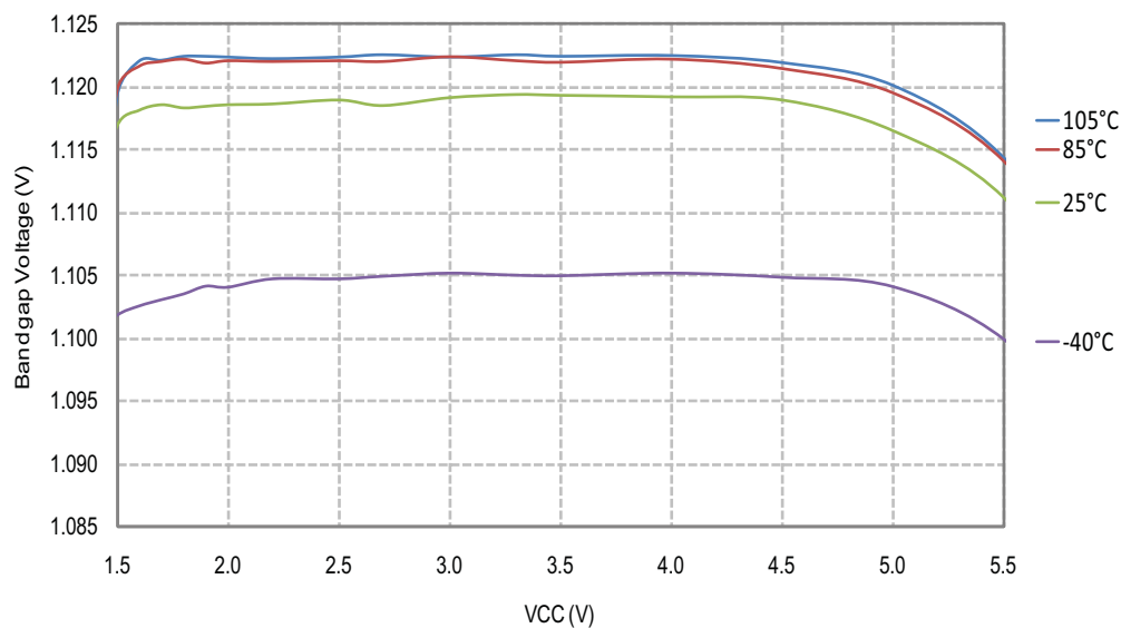
Figure 31-79. ATmega168PB: Calibrated Bandgap Voltage vs. Vcc
