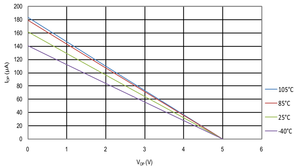
Figure 31-15. ATmega48PB/88PB: I/O Pin Pull-up Resistor Current vs. Input Voltage ( V_{CC} = 5V )
