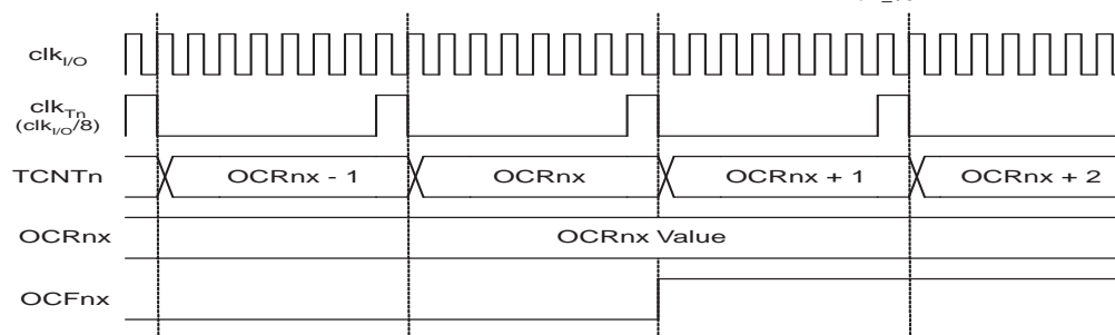
Figure 19-10. Timer/Counter Timing Diagram, Setting of \text{OCF2A} , with Prescaler ( f_{\text{clk}_{I/O}}/8 )
