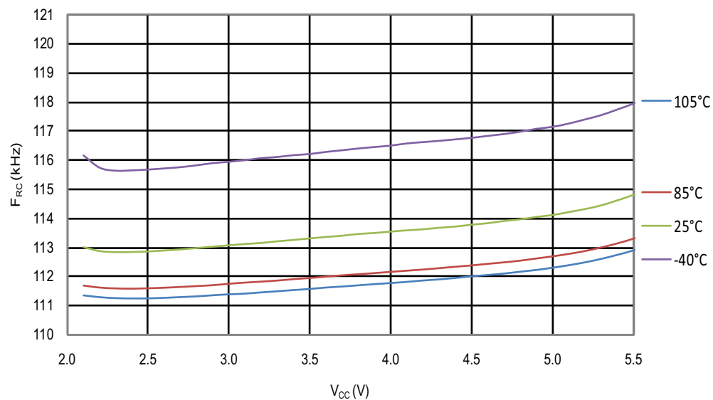
Figure 31-35. ATmega48PB/88PB: Watchdog Oscillator Frequency vs. V_{CC}
