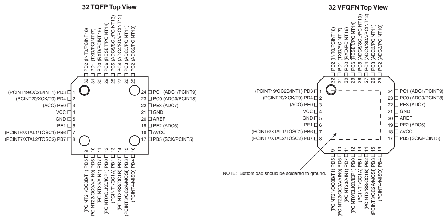
Figure 2-1. Pinout ATmega48PB/88PB/168PB
