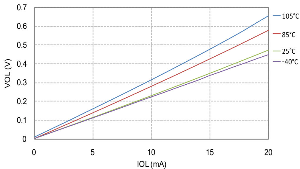
Figure 31-66. ATmega168PB: I/O Pin Output Voltage vs. Sink Current ( V_{CC} = 5V )
