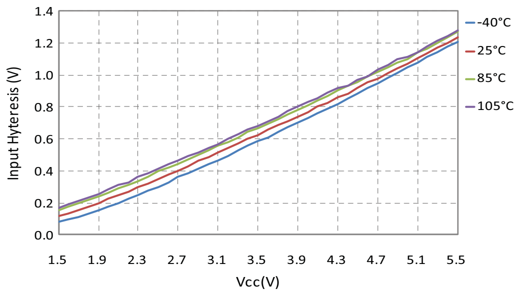
Figure 31-71. ATmega168PB I/O Pin Input Hysteresis vs. V_{CC}
