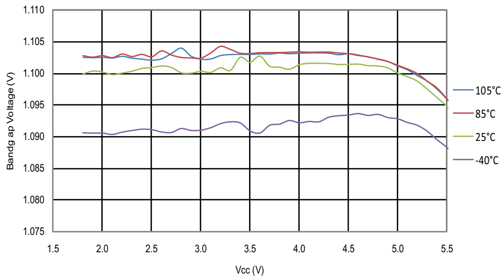
Figure 31-33. ATmega48PB/88PB: Calibrated Bandgap Voltage vs. Vcc
