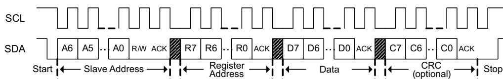
Figure 7-4. I 2 C Write
