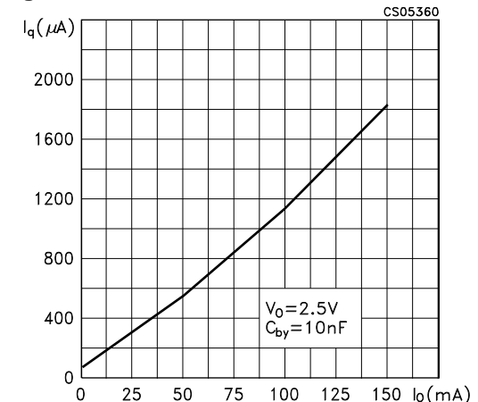
Figure 6. Quiescent current vs. load current
