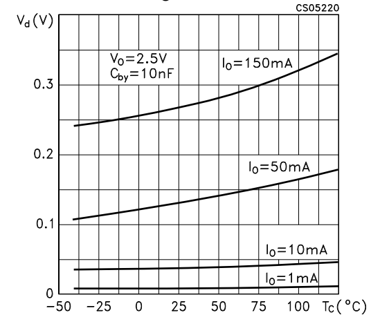
Figure 4. Dropout voltage vs. temperature ( V_O = 2.5\text{ V} )
