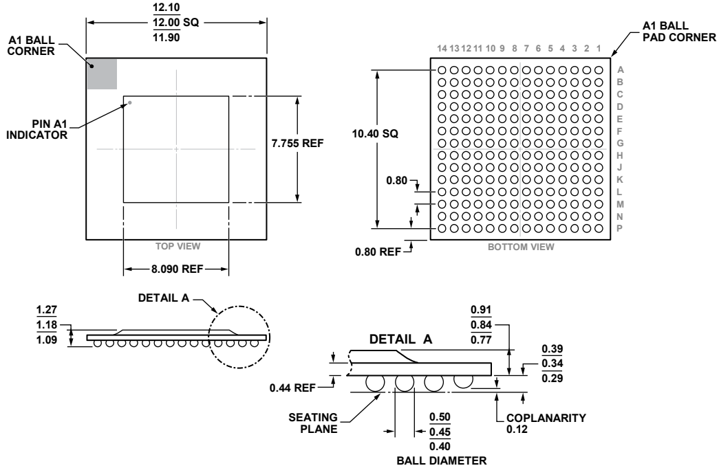
COMPLIANT TO JEDEC STANDARDS MO-275-GGAB-1. Figure 466. 196-Ball Chip Scale Package Ball Grid Array [CSP_BGA] (BC-196-13) Dimensions shown in millimeters
