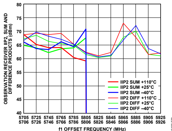
Figure 379. Observation Receiver IIP2, Sum and Difference Products vs. f1 Offset Frequency, Tones Separated by 1 MHz Swept Across Pass Band at -19 dBm Each, LO = 5700 MHz, Attenuation = 0 dB
