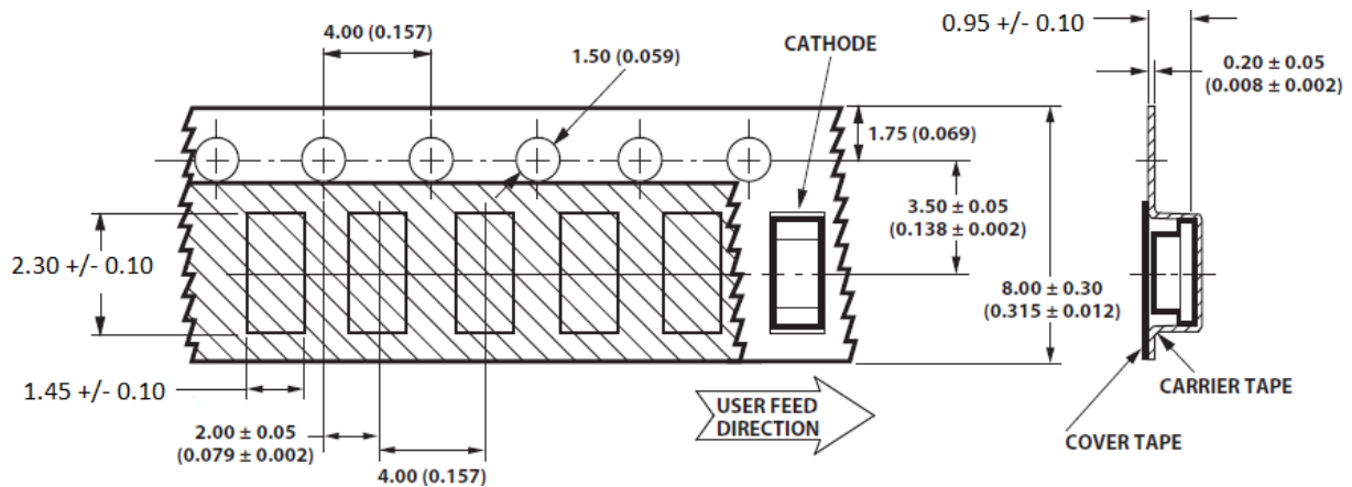
Figure 14. Tape dimensions
