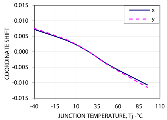
Figure 7. Chromaticity shift vs Temperature
