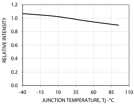
Figure 6. Relative intensity vs Temperature
