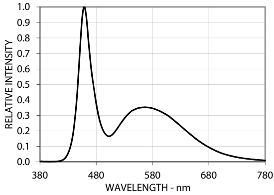
Figure 2. Spectrum
