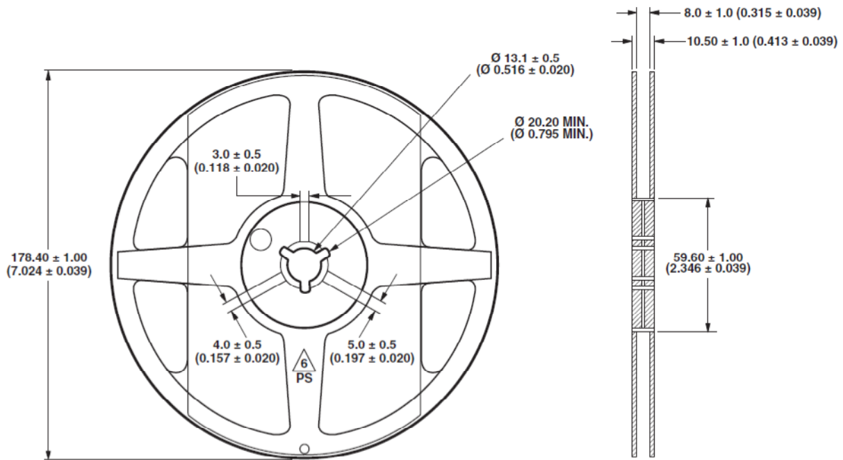
Figure 13. Reel dimensions
