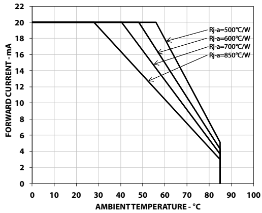
Figure 10. Derating curve
