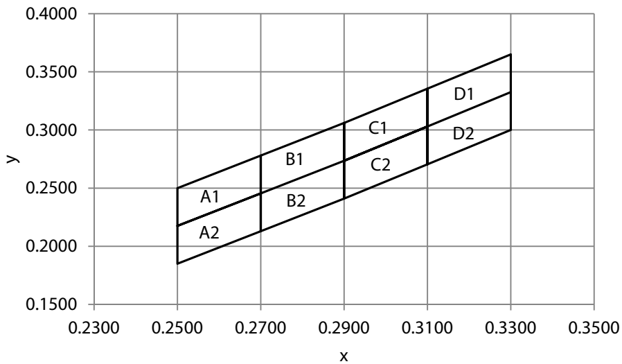
Figure 1. Chromaticity diagram
