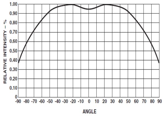
Figure 9. Radiation pattern
