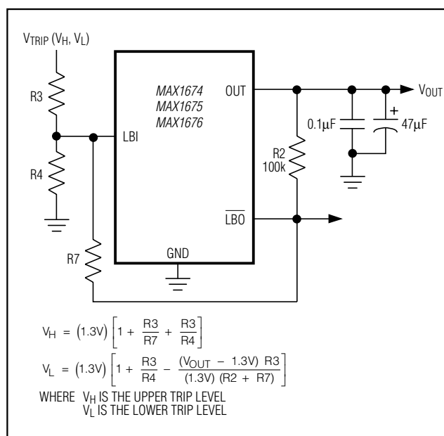
Figure 9. Adding External Hysteresis to the Low-Battery Indicator
