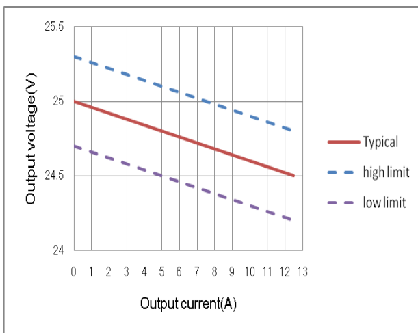
Figure 5: Output voltage vs. Output current @ Vin=72V. Droop function.
