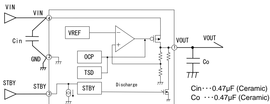
Fig. 2 Block Diagrams
