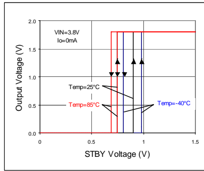
Fig 10. STBY Threshold
