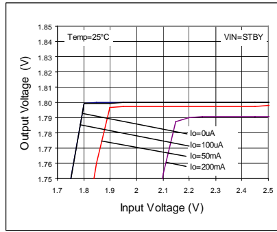
Fig 4. Line Regulation
