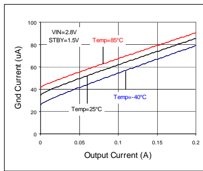
Fig 7. IOUT - IGND
