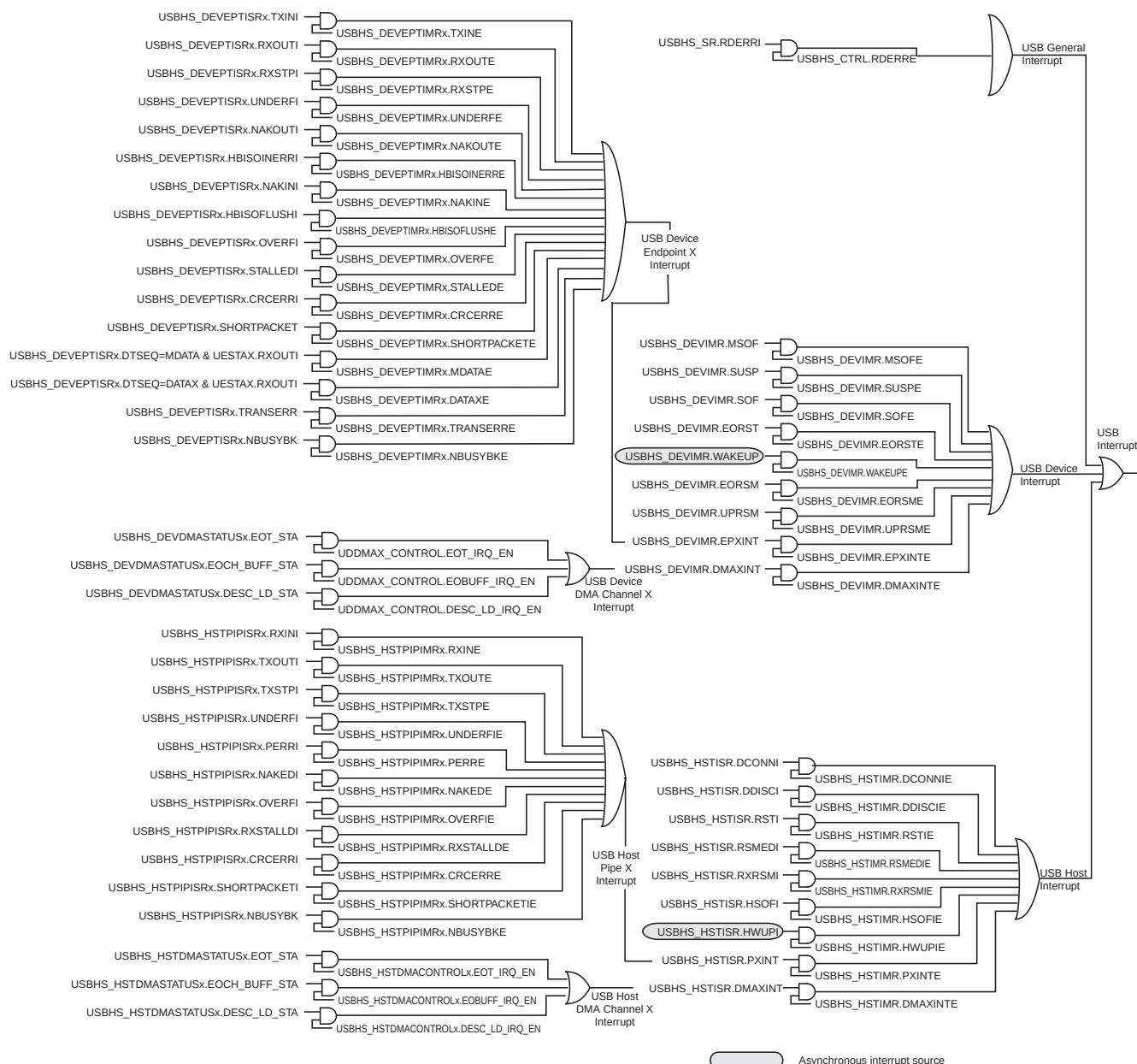
Figure 36-3. Interrupt System
