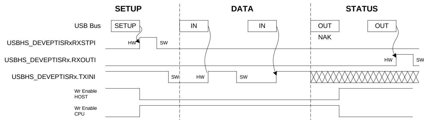
Figure 36-10. Control Read
