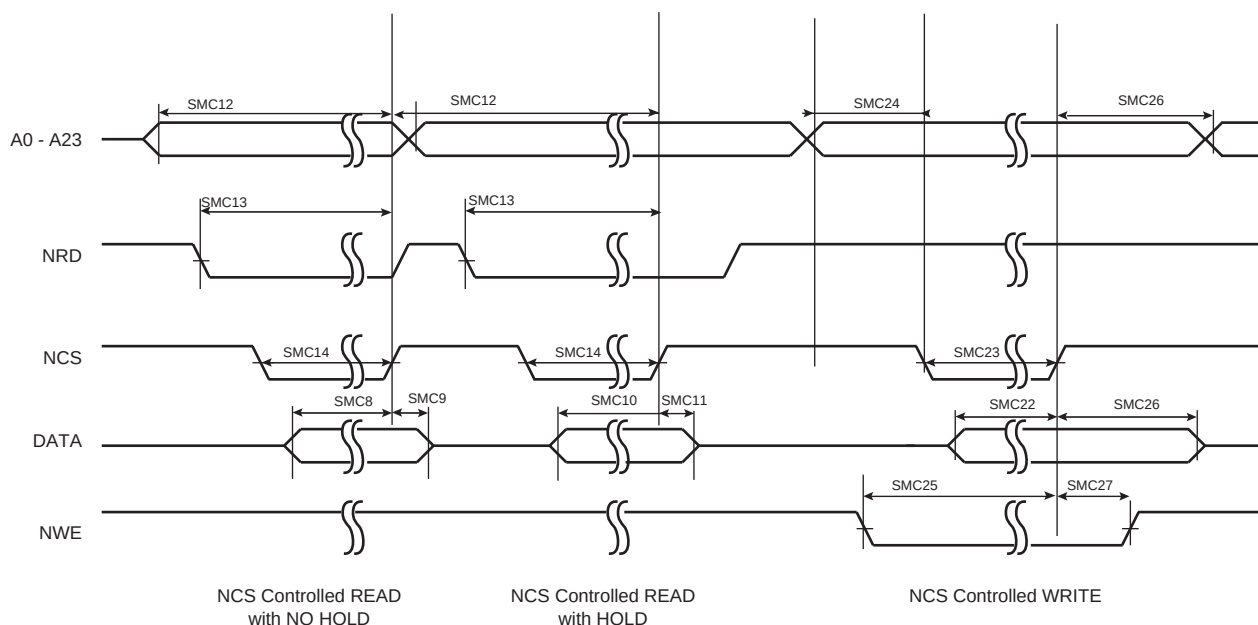
Figure 54-23. SMC Timings - NCS Controlled Read and Write
