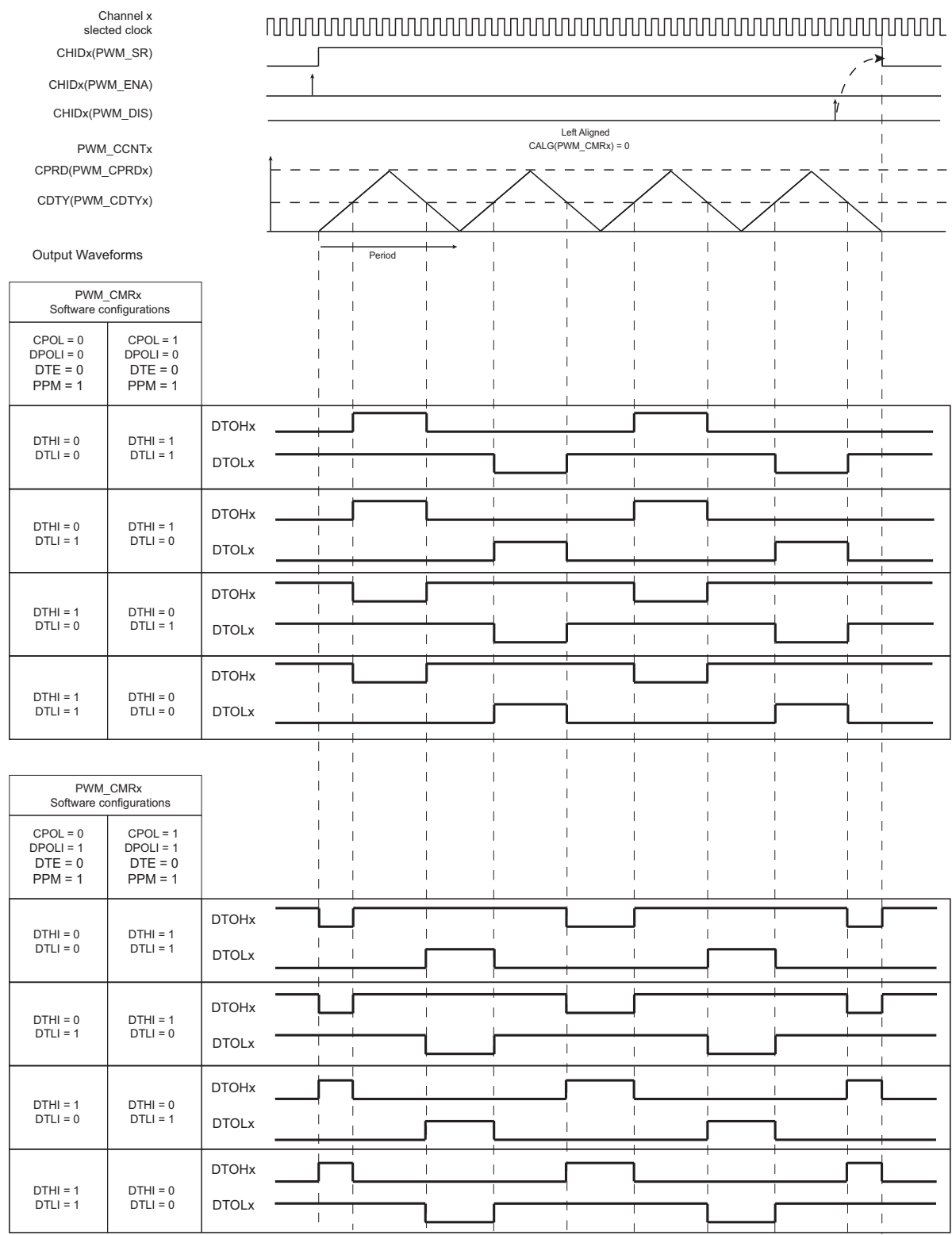
Figure 47-12. PWM Push-Pull Waveforms: Center-Aligned Mode
