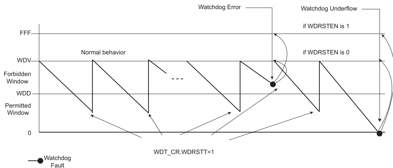
Figure 22-2. Watchdog Behavior
