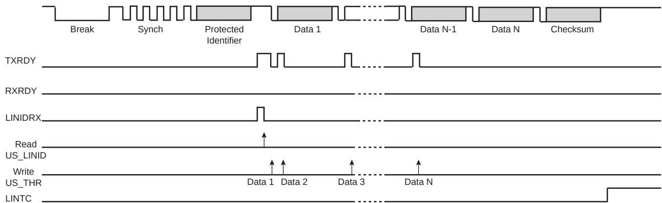
Figure 43-48. Slave Node Configuration, NACT = PUBLISH
