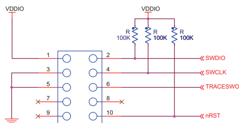
Figure 56-1. SWD Schematic Example with a 10-pin Connector
