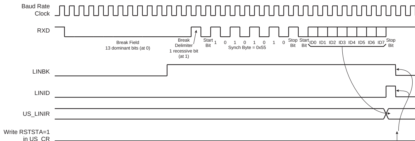
Figure 43-40. Header Reception
