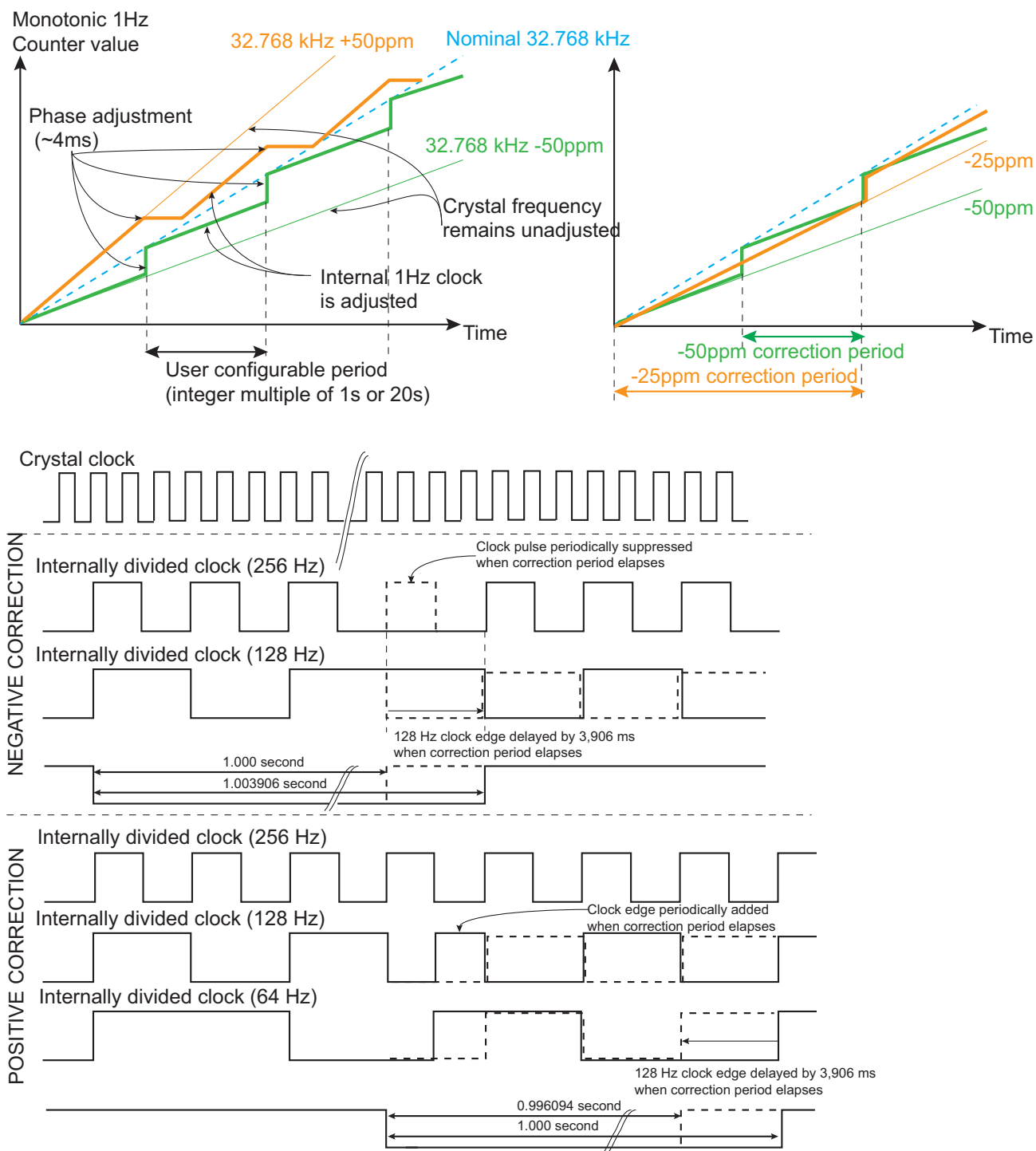
Figure 25-4. Calibration Circuitry Waveforms
