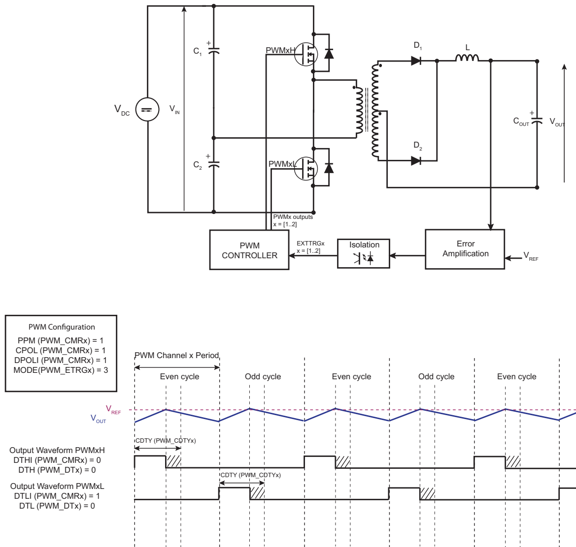
Figure 47-14. Half-Bridge Converter Application: Feedback Regulation
