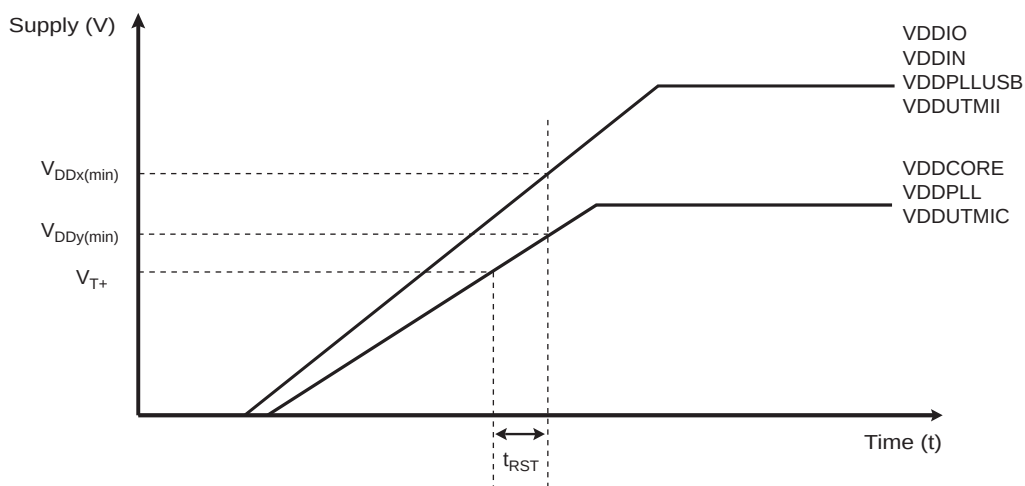
Figure 5-1. Power-up Sequence
