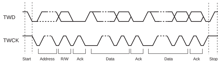
Figure 41-3. Transfer Format
