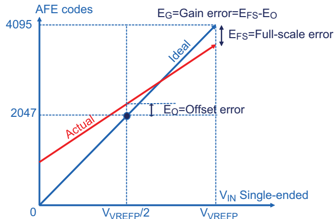
Figure 54-14. Gain and Offset Errors in Single-ended Mode
