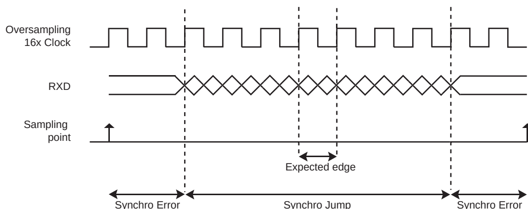
Figure 43-60. Bit Resynchronization
