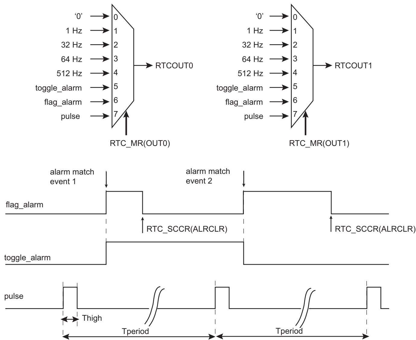
Figure 25-5. Waveform Generation
