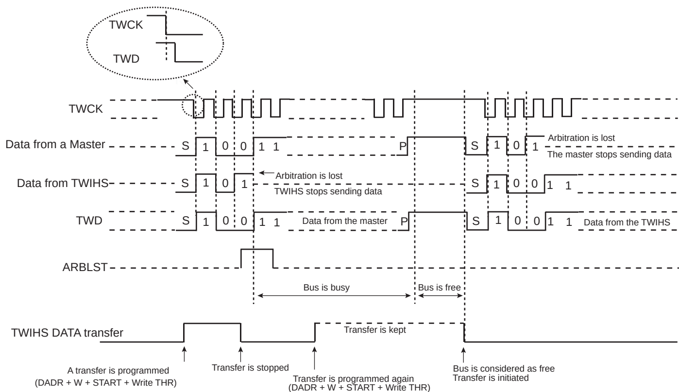
Figure 41-29. Arbitration Cases
