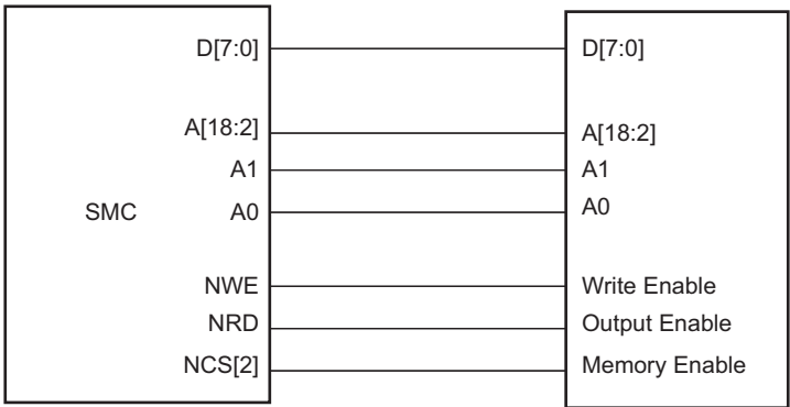
Figure 33-2. Memory Connection for an 8-bit Data Bus
