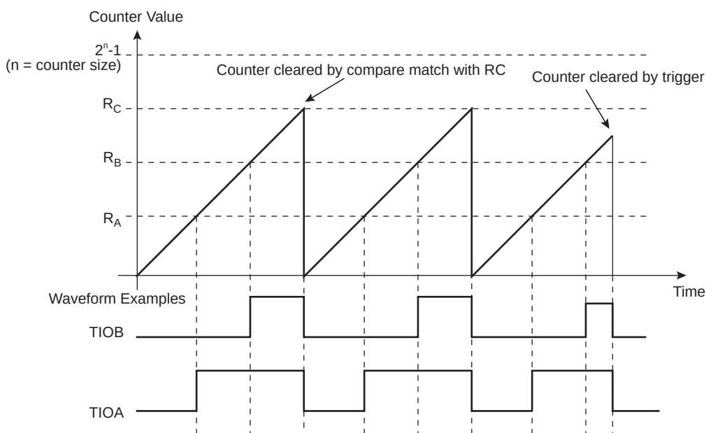
Figure 46-11. WAVSEL = 10 with Trigger
