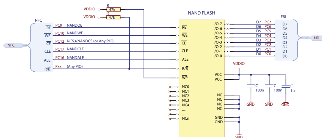
Figure 56-5. Schematic Example with a 2 Gb/8-bit NAND Flash
