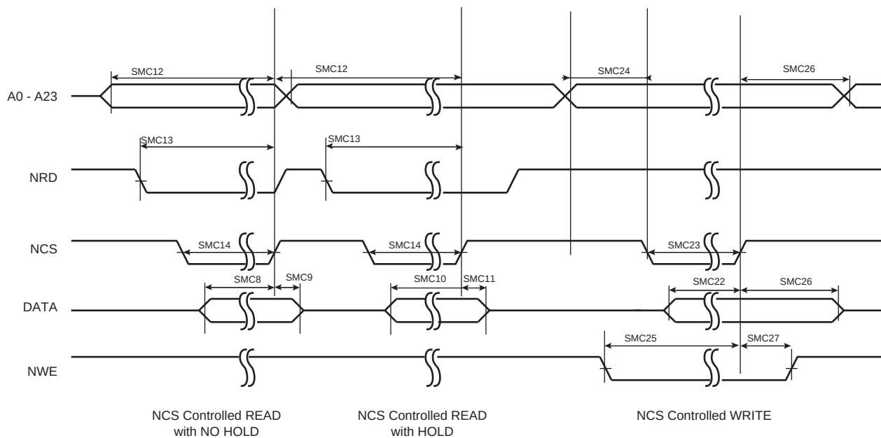
Figure 54-48. SMC Timings - NCS Controlled Read and Write
