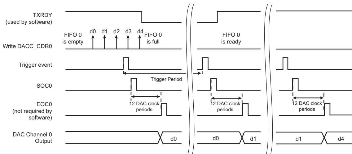
Figure 49-2. Conversion Sequence in External Trigger Mode
