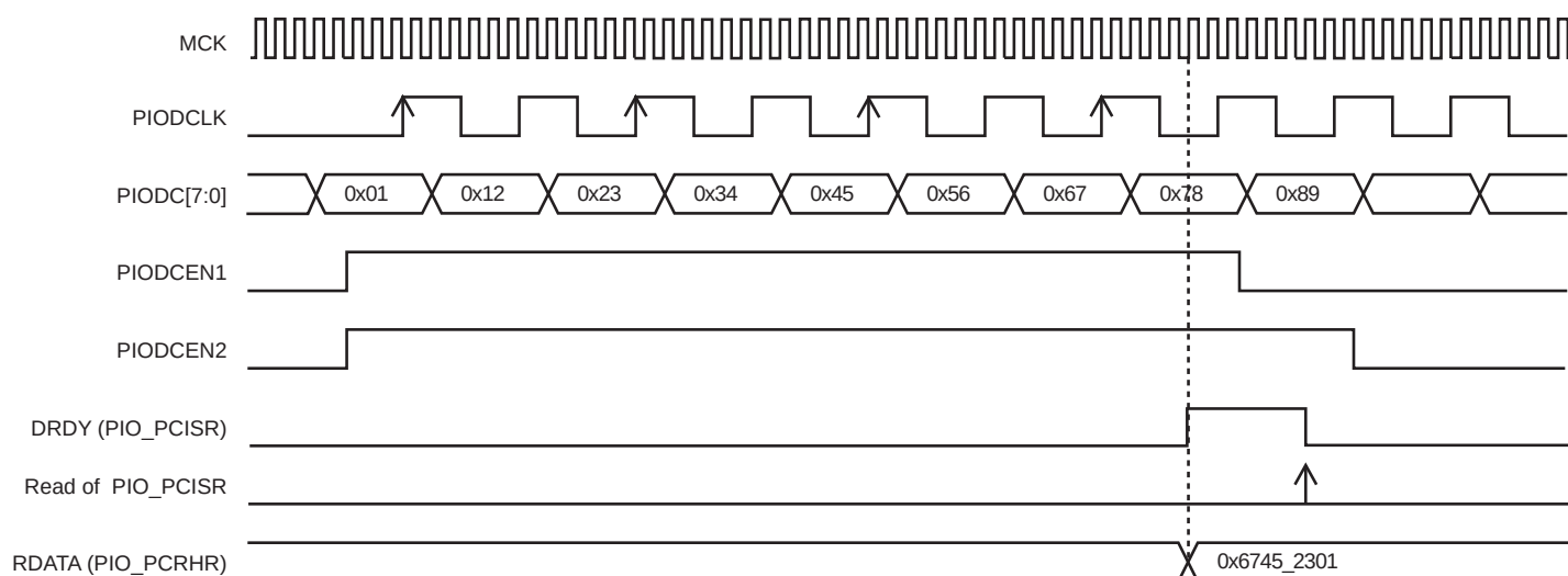
Figure 30-12. Parallel Capture Mode Waveforms (DSIZE = 2, ALWYS = 0, HALFS = 1, FRSTS = 1)
