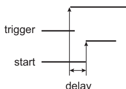
Figure 48-6. Conversion Start with the Hardware Trigger
