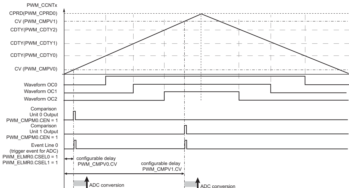
Figure 47-26. Event Line Generation Waveform (Example)
