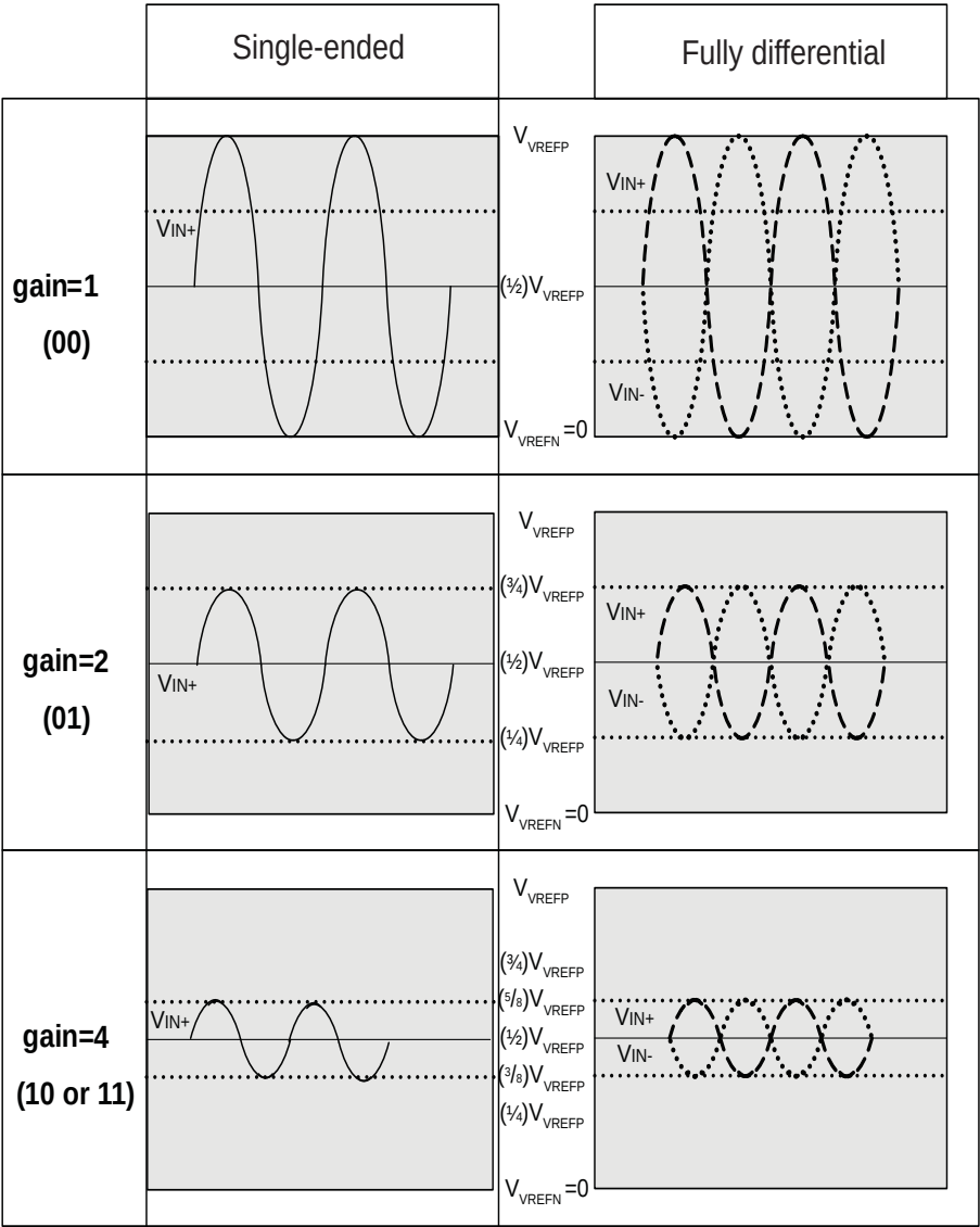
Figure 48-7. Analog Full Scale Ranges in Single-Ended/Differential Applications Versus Gain
