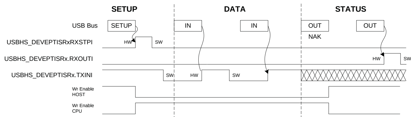
Figure 36-10. Control Read
