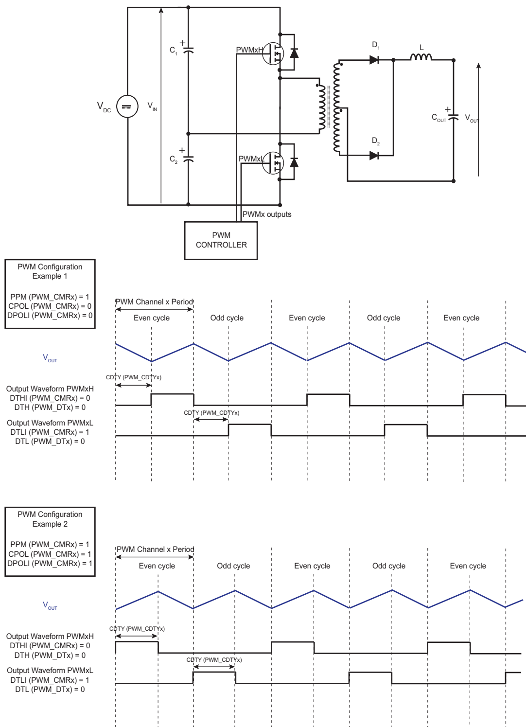
Figure 47-13. Half-Bridge Converter Application: No Feedback Regulation
