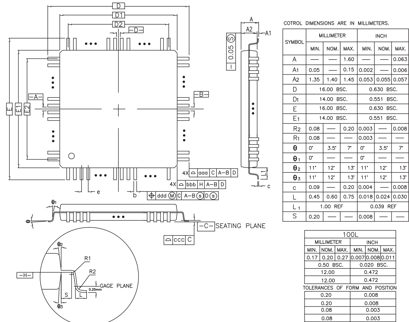
Figure 55-3. 100-pin LQFP Package Mechanical Drawing
