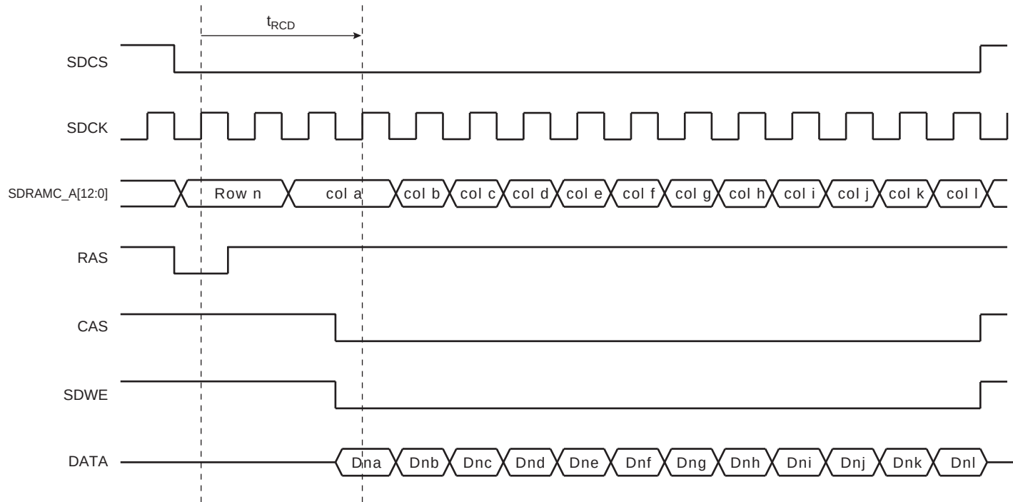
Figure 32-2. Write Burst SDRAM Access
