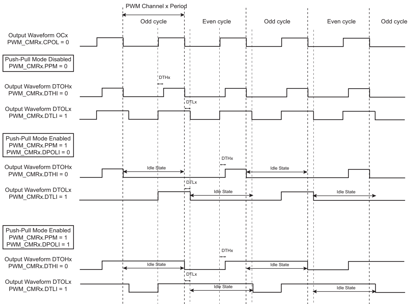
Figure 47-10. PWM Push-Pull Mode
