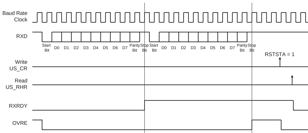
Figure 43-20. Receiver Status
