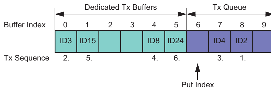
Figure 45-11. Example of Mixed Configuration Dedicated Tx Buffers / Tx Queue
