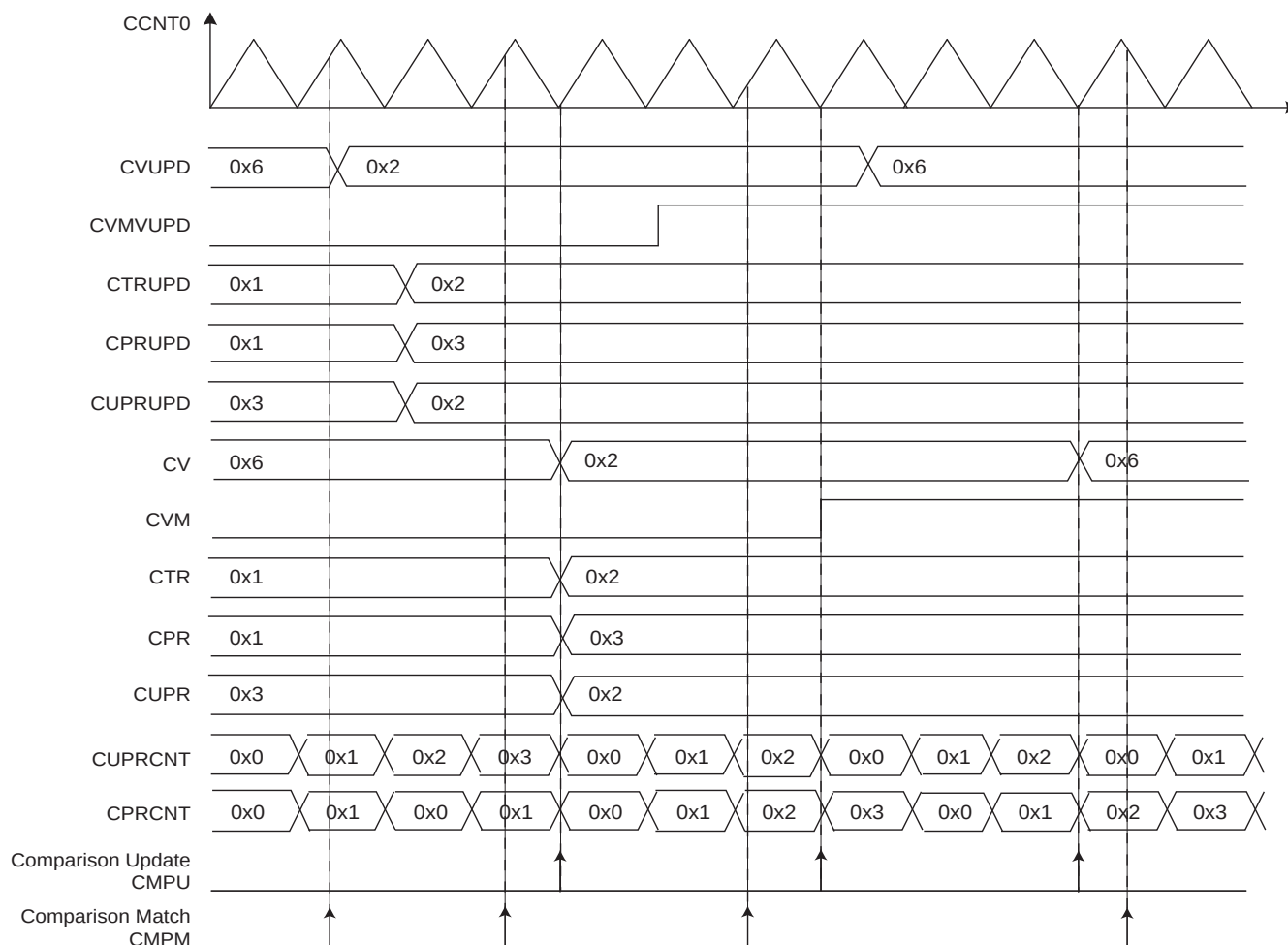
Figure 47-24. Comparison Waveform
