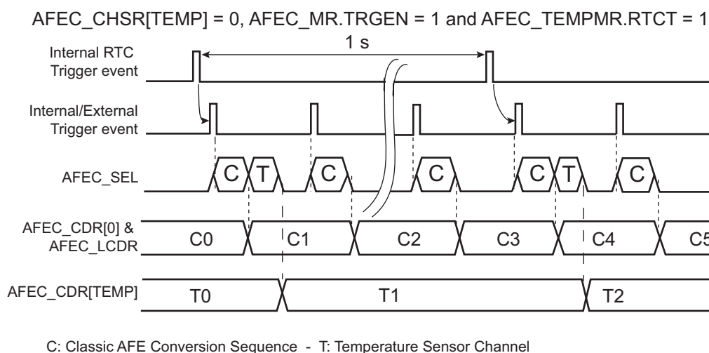
Figure 48-9. Optimized Temperature Conversion Combined with Classical Conversions
