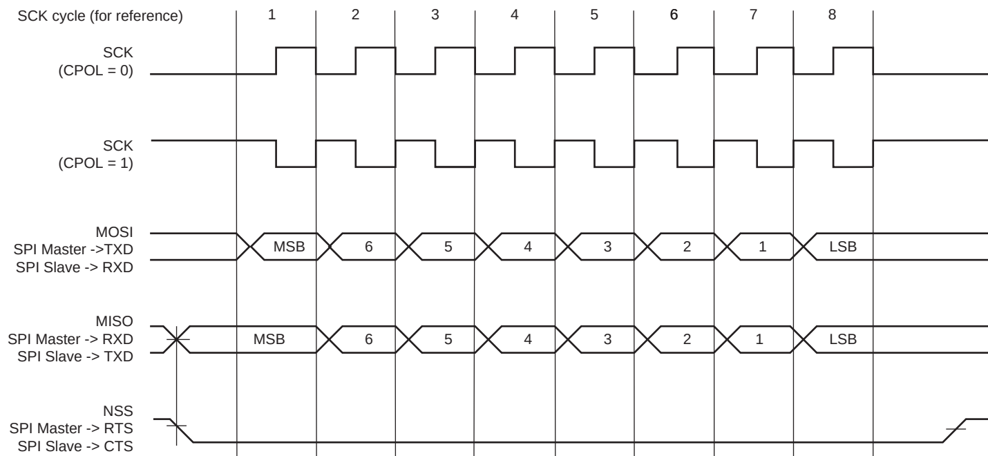
Figure 43-37. SPI Transfer Format (CPHA = 1, 8 bits per transfer)
