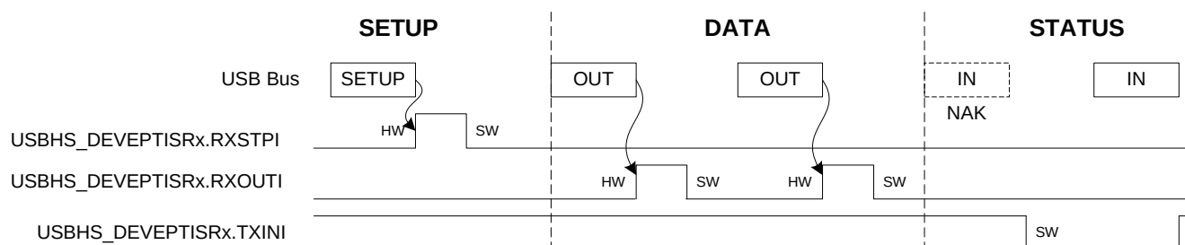
Figure 36-9. Control Write
