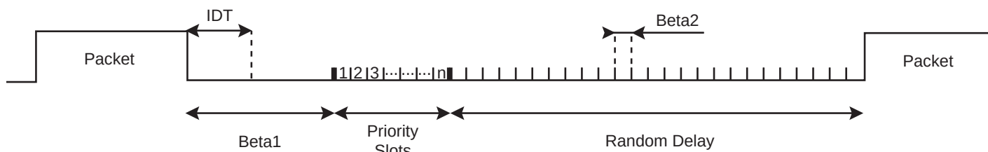
Figure 43-59. LON timings
