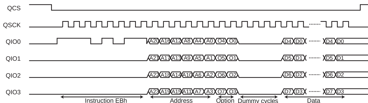
Figure 39-8. Instruction Frame
