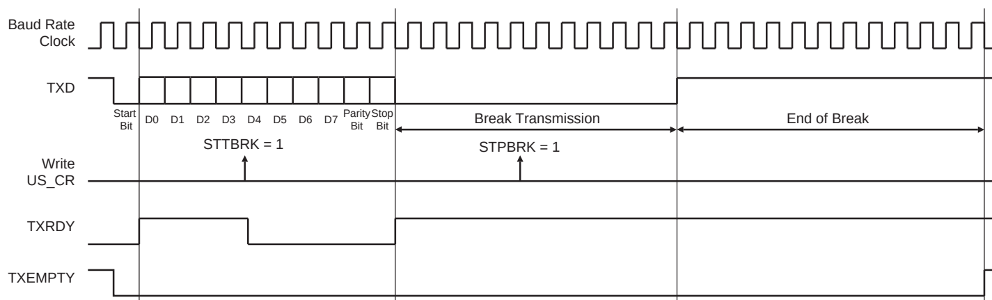
Figure 43-25. Break Transmission
