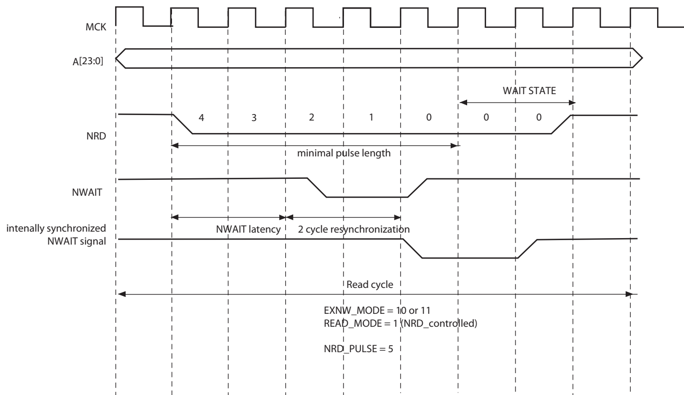
Figure 33-29. NWAIT Latency
