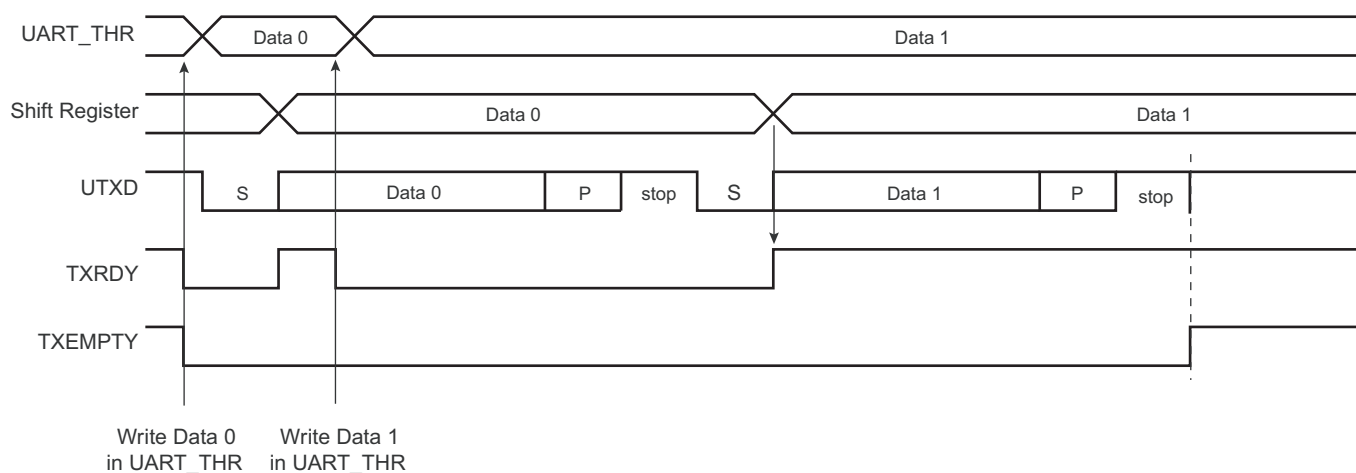
Figure 44-11. Transmitter Control
