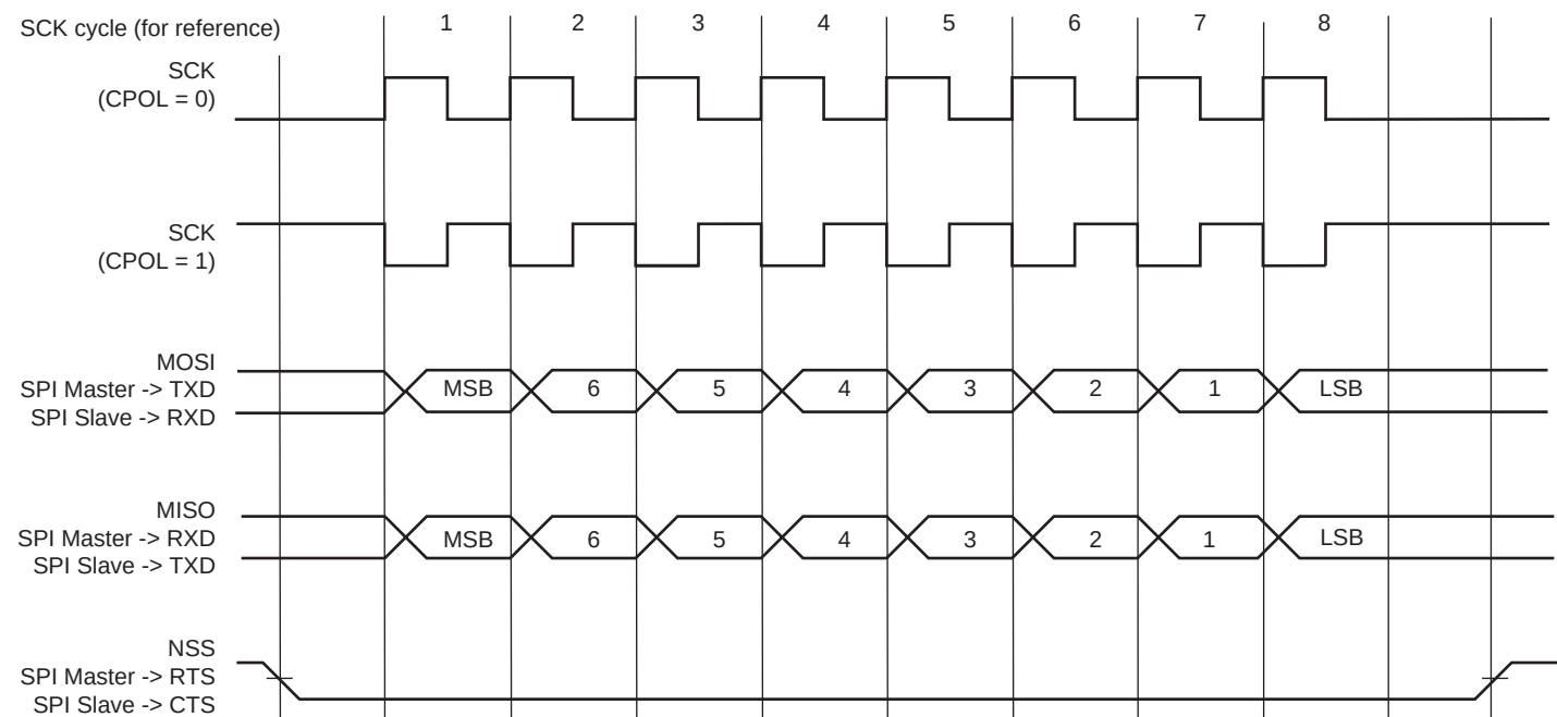
Figure 43-38. SPI Transfer Format (CPHA = 0, 8 bits per transfer)
