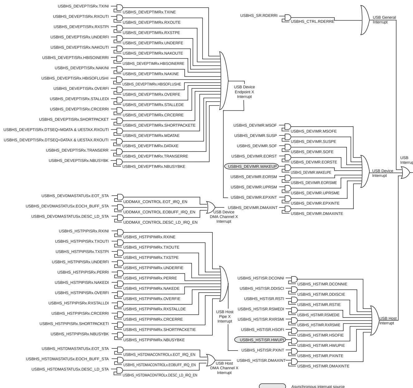
Figure 36-3. Interrupt System
