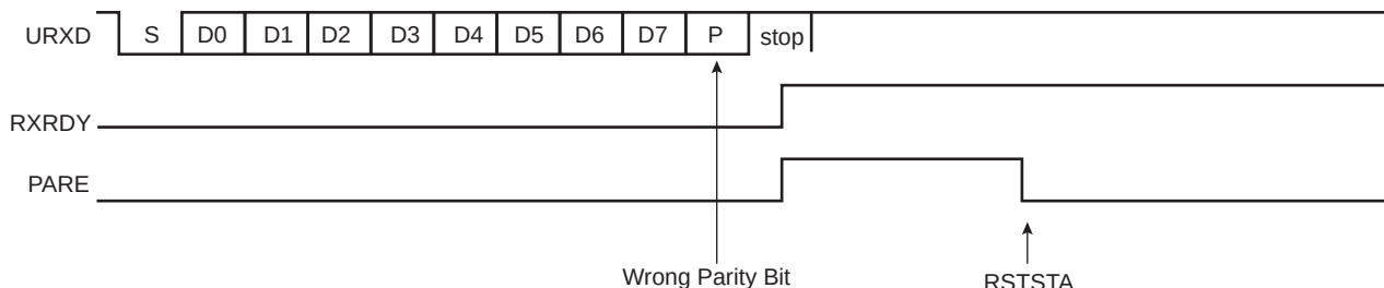
Figure 44-8. Parity Error
