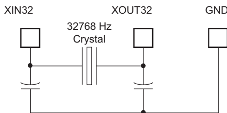
Figure 28-2. Typical 32.768 kHz Crystal Oscillator Connection
