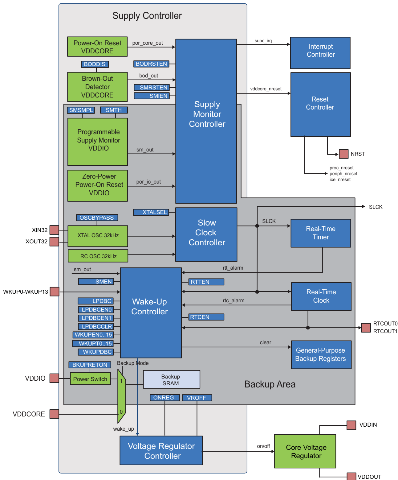
Figure 21-1. Supply Controller Block Diagram
