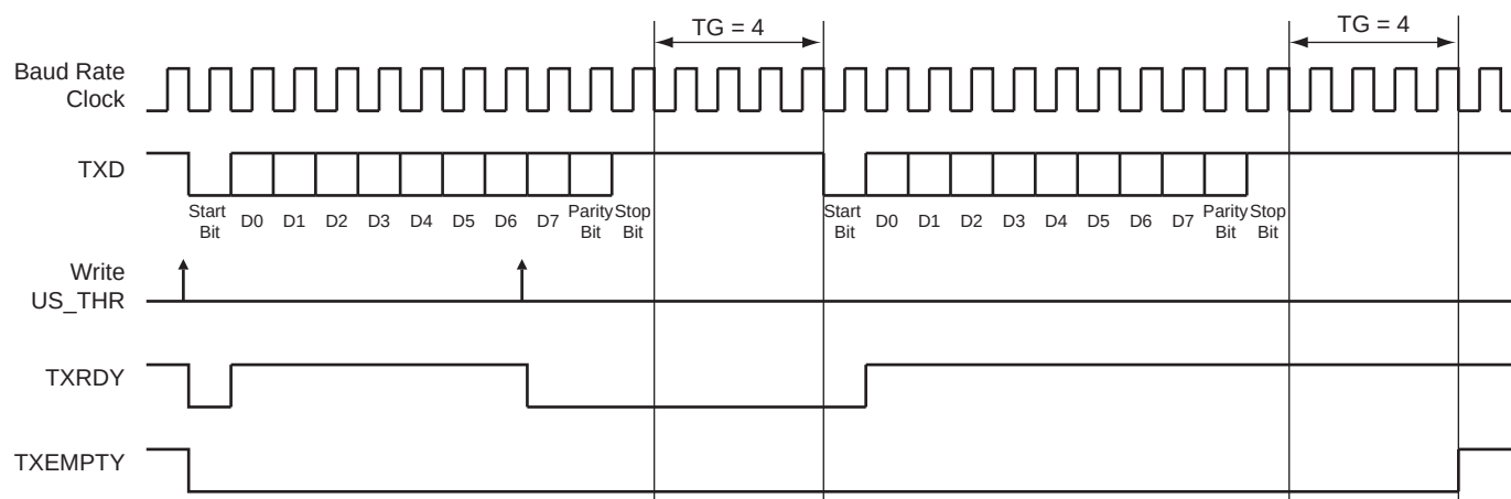
Figure 43-22. Timeguard Operations
