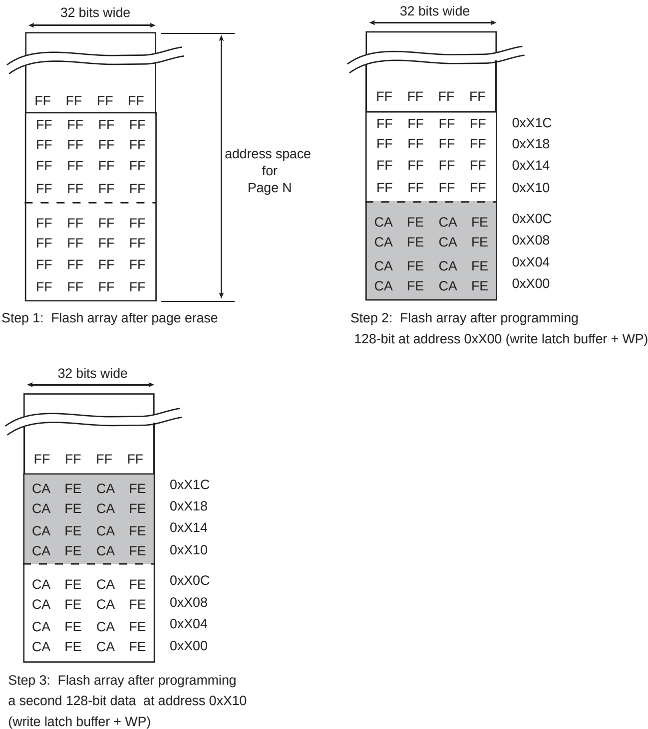
Figure 20-9. Partial Page Programming
