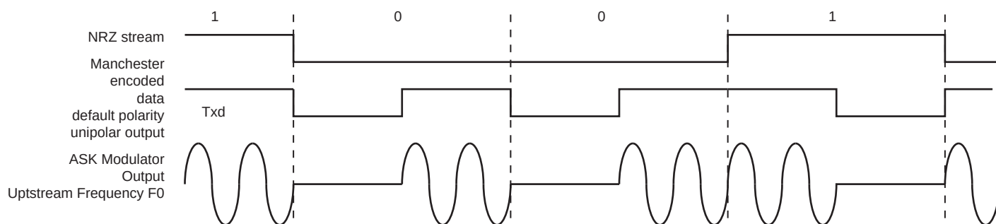
Figure 43-17. ASK Modulator Output
