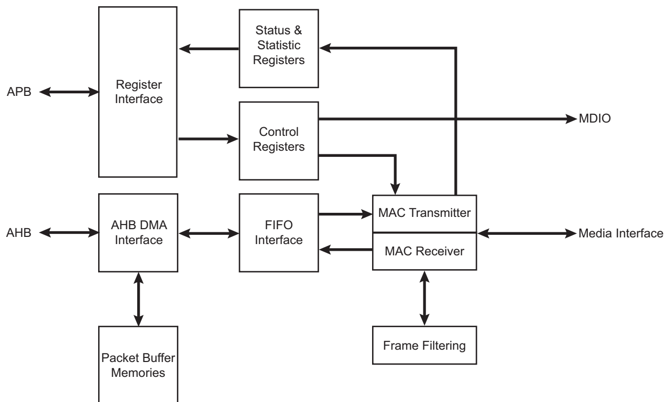
Figure 37-1. Block Diagram
