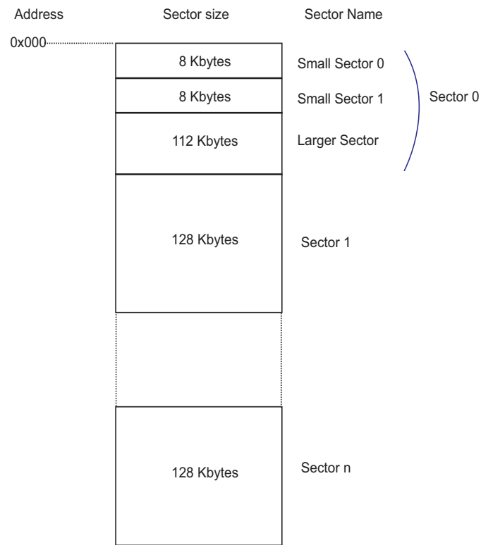
Figure 9-1. Global Flash Organization
