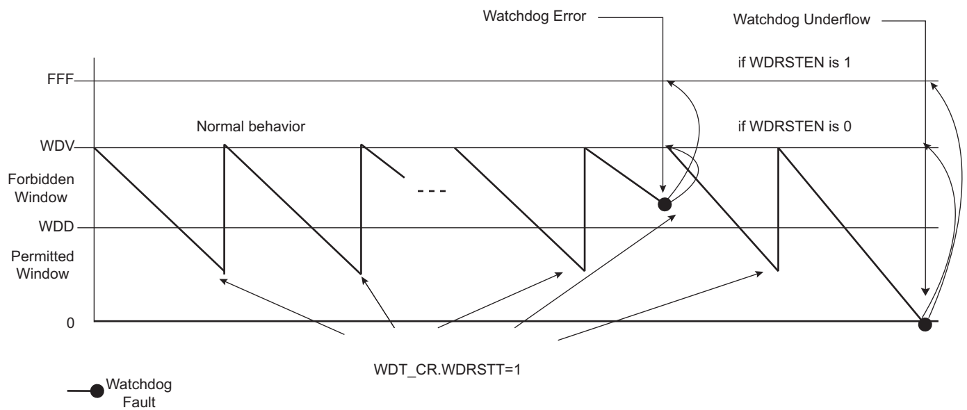
Figure 22-2. Watchdog Behavior
