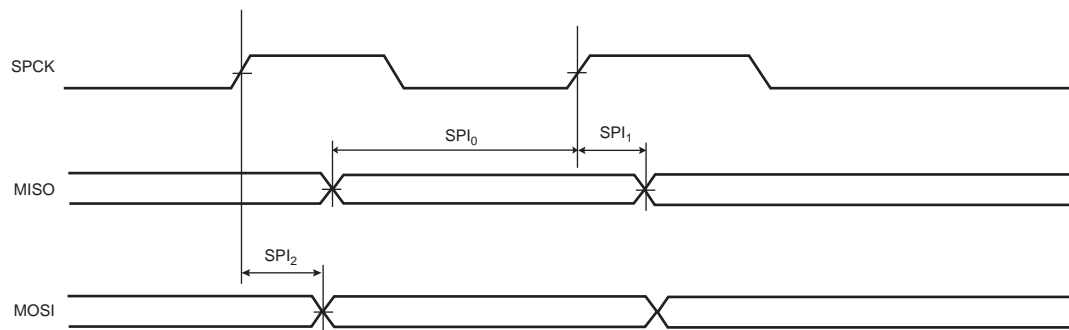
Figure 54-19. SPI Master Mode with (CPOL= NCPHA = 0) or (CPOL= NCPHA= 1)
