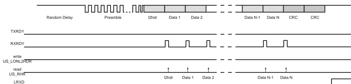
Figure 43-62. Rx Frame
