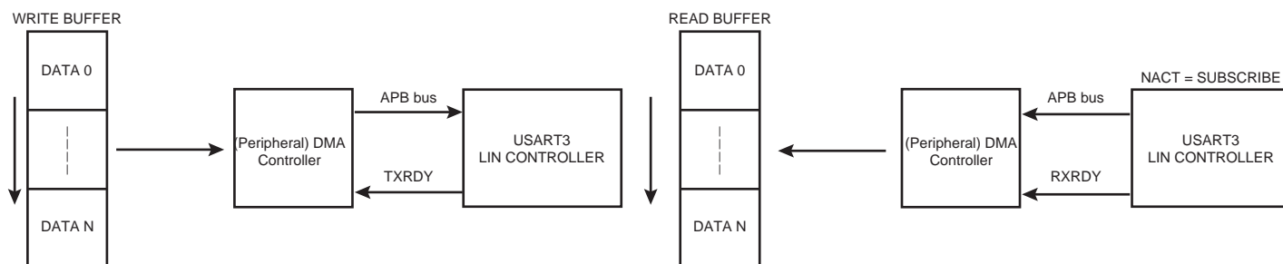
Figure 43-53. Slave Node with DMAC
