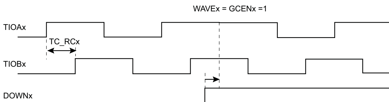
Figure 46-22. 2-bit Gray Up/Down Counter
