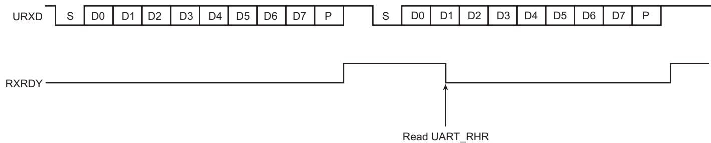
Figure 44-6. Receiver Ready
