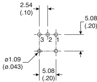
P.C. Mounting
