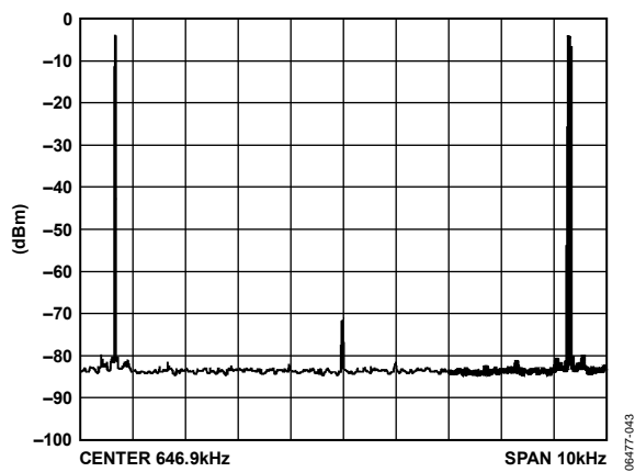
Figure 19. MTPR at 647 kHz
