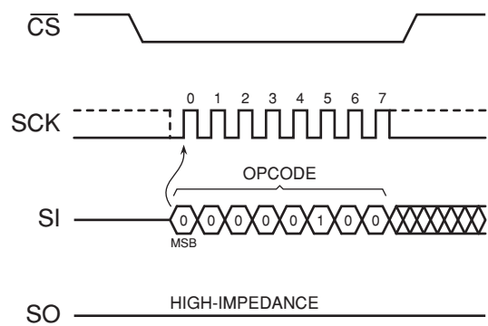
Figure 9-2. Write Disable
