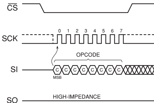
Figure 8-6. Chip Erase
