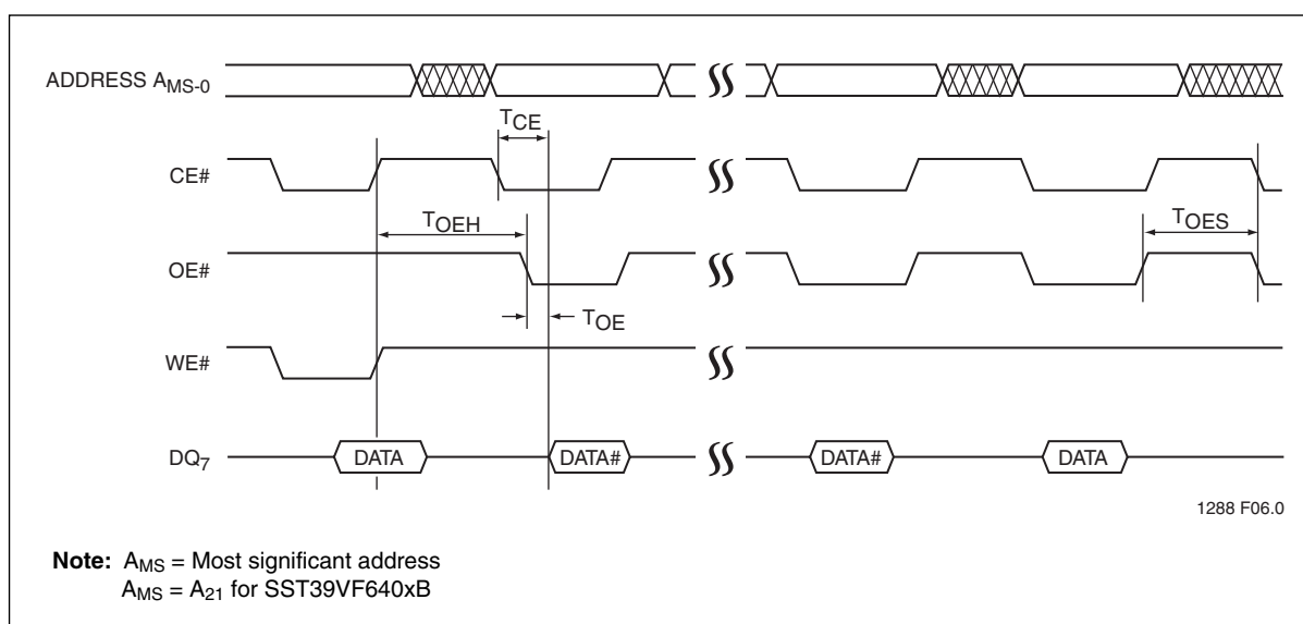
Figure 6: Data# Polling Timing Diagram
