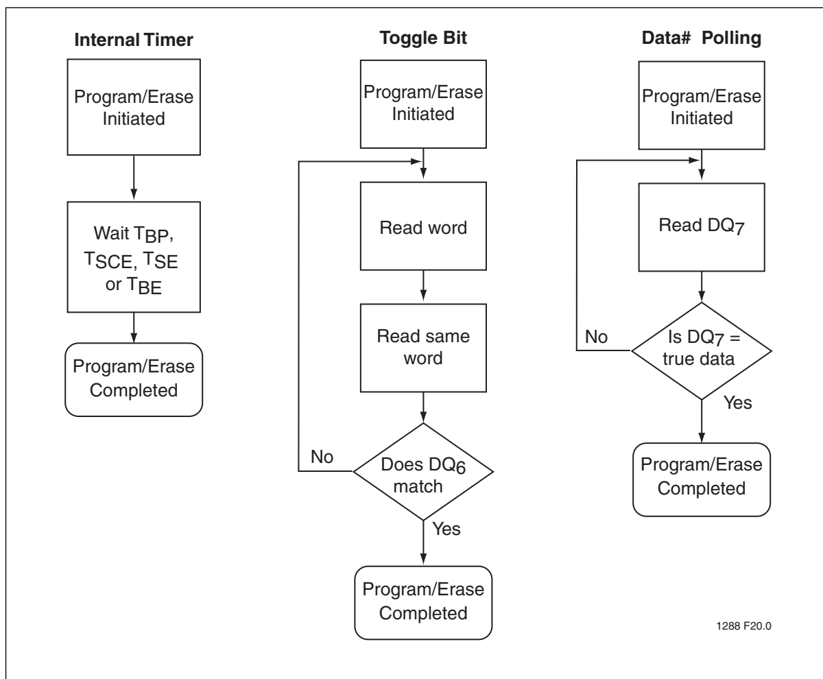
Figure 20: Wait Options
