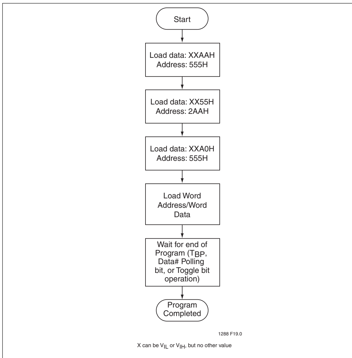
Figure 19: Word-Program Algorithm
