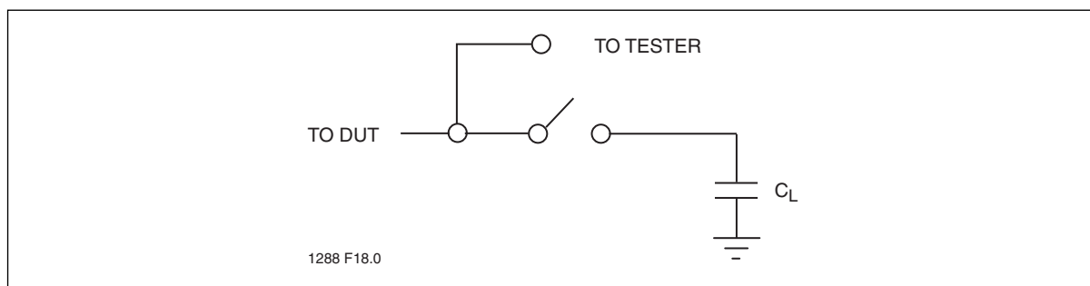
Figure 18: A Test Load Example
