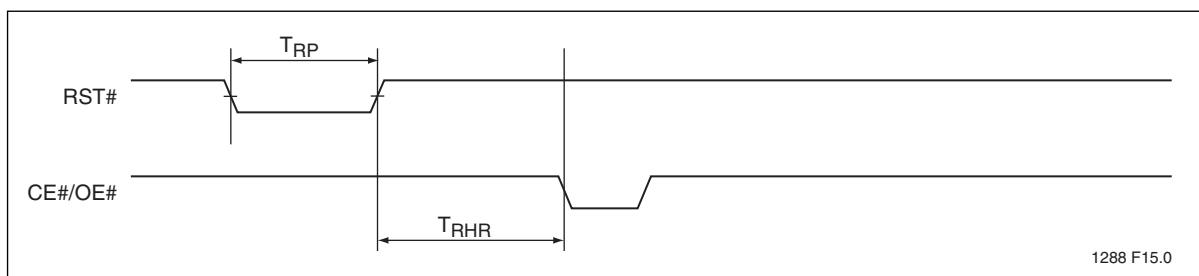
Figure 15: RST# Timing Diagram (When no internal operation is in progress)
