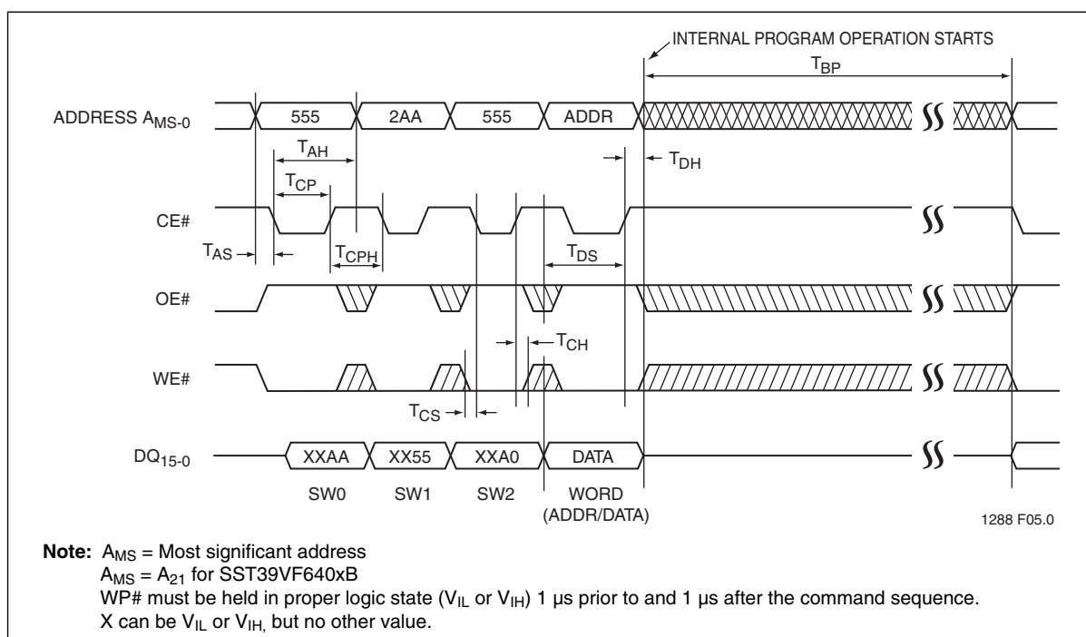
Figure 5: CE# Controlled Program Cycle Timing Diagram
