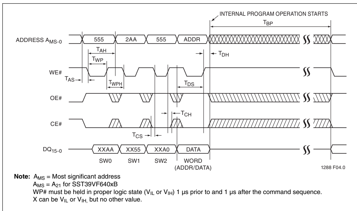
Figure 4: WE# Controlled Program Cycle Timing Diagram
