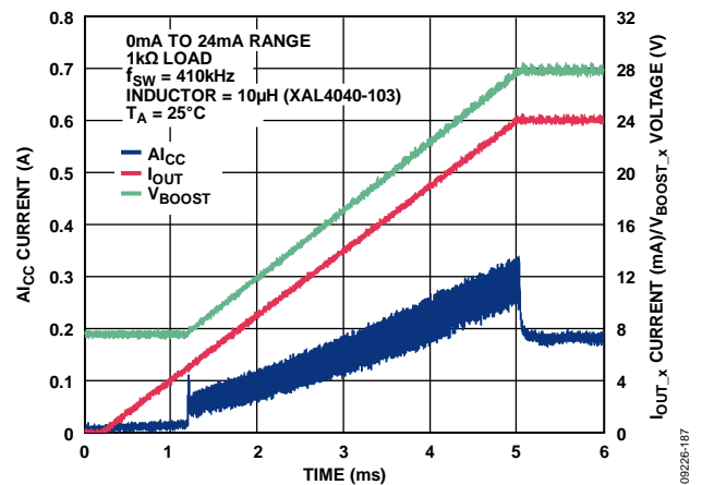
Figure 85. I_{CC} Current vs. Time for 24 mA Step Through 1 k \Omega Load with Slew Rate Control
