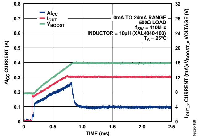
Figure 84. I_{CC} Current vs. Time for 24 mA Step Through 500 \Omega Load with External 51 k \Omega Compensation Resistor
