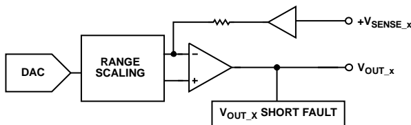
Figure 72. Voltage Output
