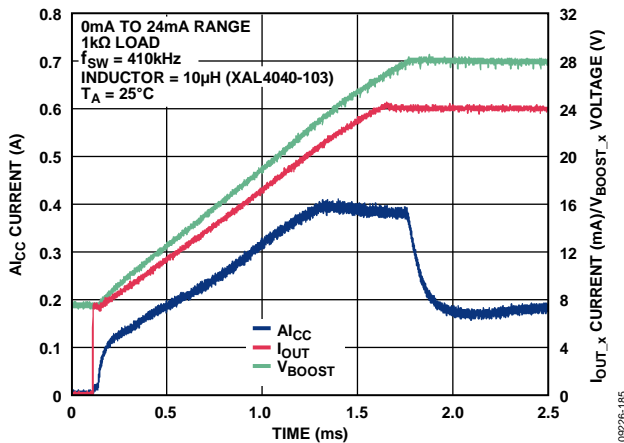
Figure 83. I_{CC} Current vs. Time for 24 mA Step Through 1 k \Omega Load with External 51 k \Omega Compensation Resistor
