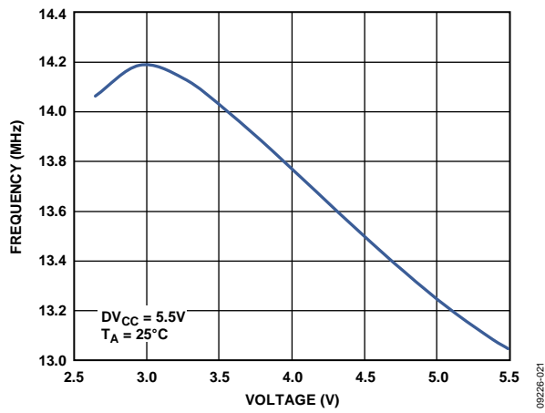
Figure 70. Internal Oscillator Frequency vs. DV CC Supply Voltage
