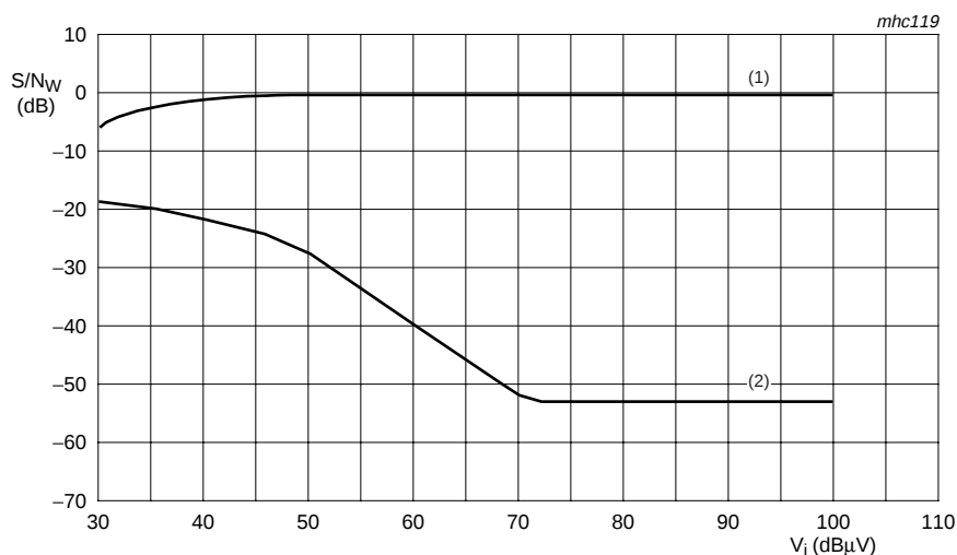
Condition: m = 54 %. (1) Signal. (2) Noise.
