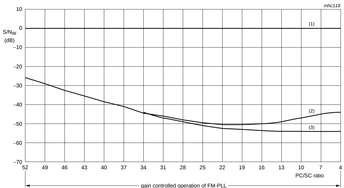
Conditions: PC / SC ratio measured at pins VIF1 and VIF2; via transformer; 27 kHz FM deviation; 50 μs de-emphasis. (1) Signal. (2) Noise at H-picture ("ITU-R BS.468-4" weighted quasi peak). (3) Noise at black picture ("ITU-R BS.468-4" weighted quasi peak).
