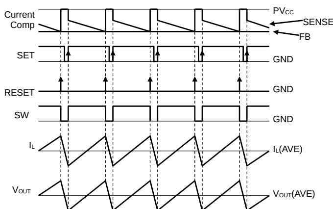
Figure 22. PWM Switching Timing Diagram
