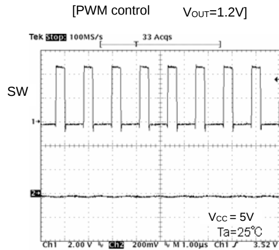
Figure 16. SW Waveform ( I_o=4\text{A} )
