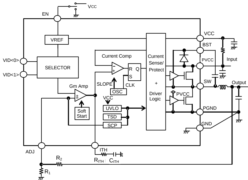
Figure 3. Block Diagram
