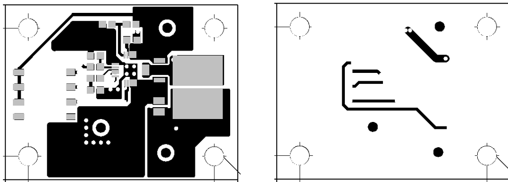
Figure 39. Layout Diagram
