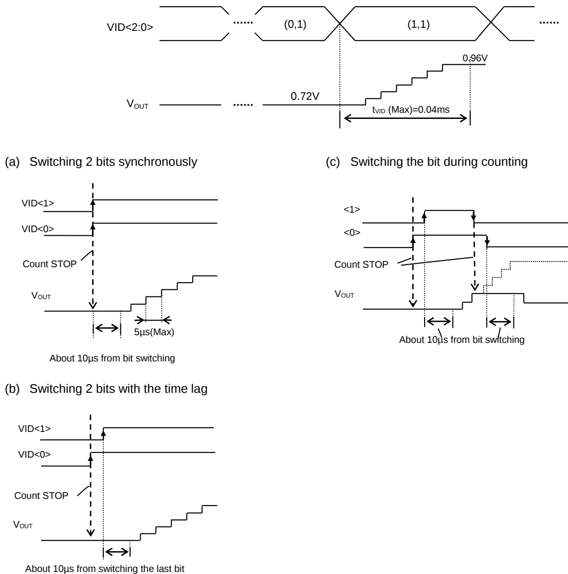
Figure 29. Timing Diagram of Setting the Output Voltage
