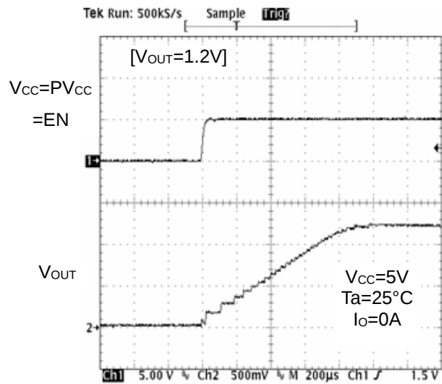
Figure 14. Soft-Start Waveform
