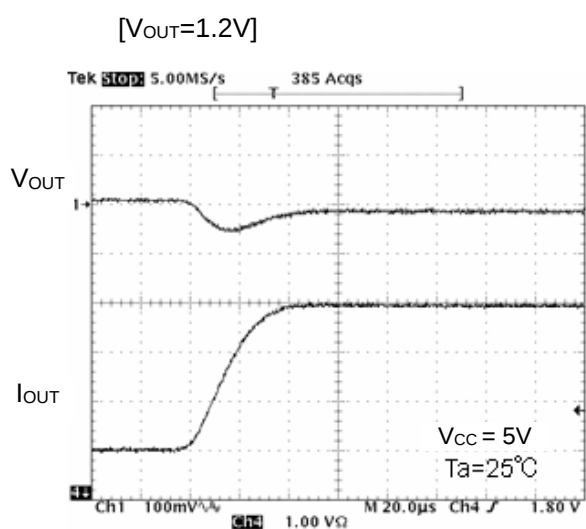
Figure 17. Transient Response ( I_o=1\text{A} to 4\text{A} , 20\mu\text{s} )
