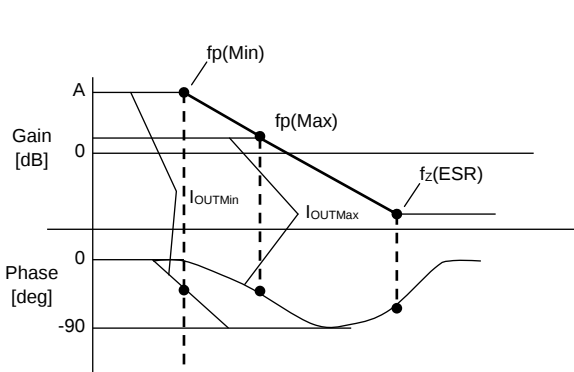
Figure 34. Open Loop Gain Characteristics
