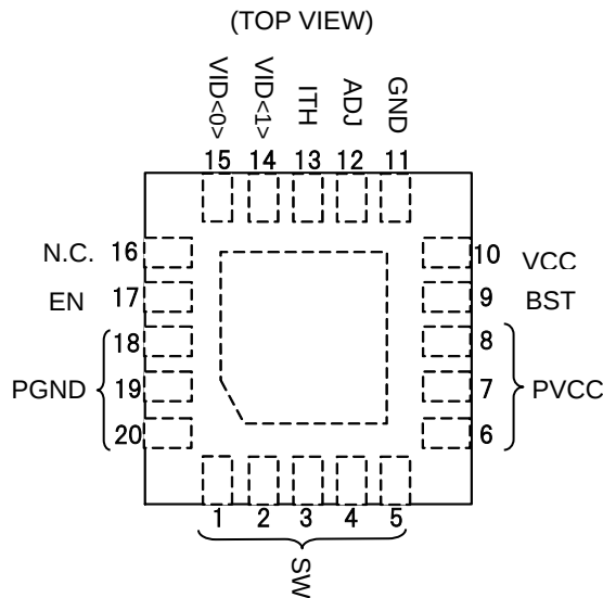
Figure 2. Pin Configuration
