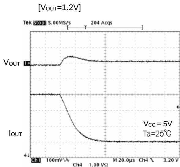
Figure 18. Transient Response (I O =4A to 1A, 20μs)
