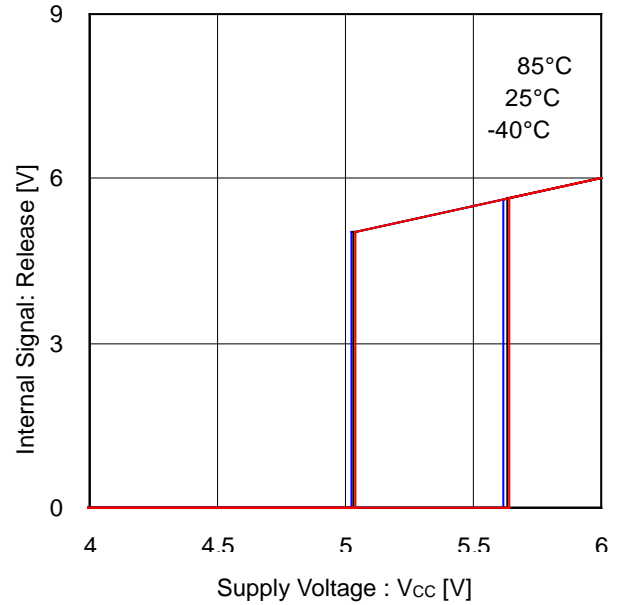
Figure 16. Internal Signal vs Supply Voltage (Under Voltage Lock Out)
