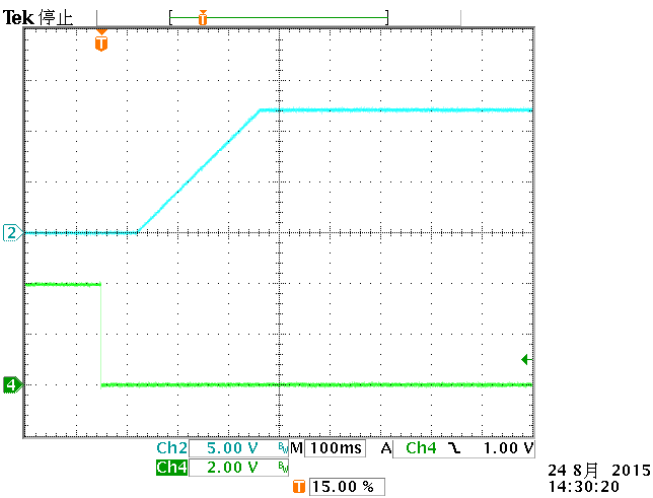
Figure 8: Turn-on transient at zero load current (10ms/div), Vin=54V; Top Trace: Vout, 5V/div; Bottom Trace: ON/OFF input, 2V/div;
