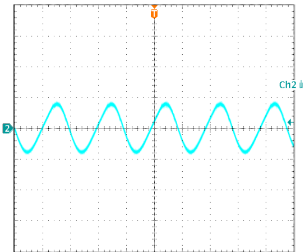
Figure 18: Output voltage ripple at nominal input voltage and rated load current (100 mV/div, 2 \mu\text{s} /div) Load capacitance: 1\mu\text{F} ceramic capacitor and 10\mu\text{F} tantalum capacitor. Bandwidth: 20 MHz. Scope measurements should be made using a BNC cable (length shorter than 20 inches). Position the load between 51 mm to 76 mm (2 inches to 3 inches) from the module.
