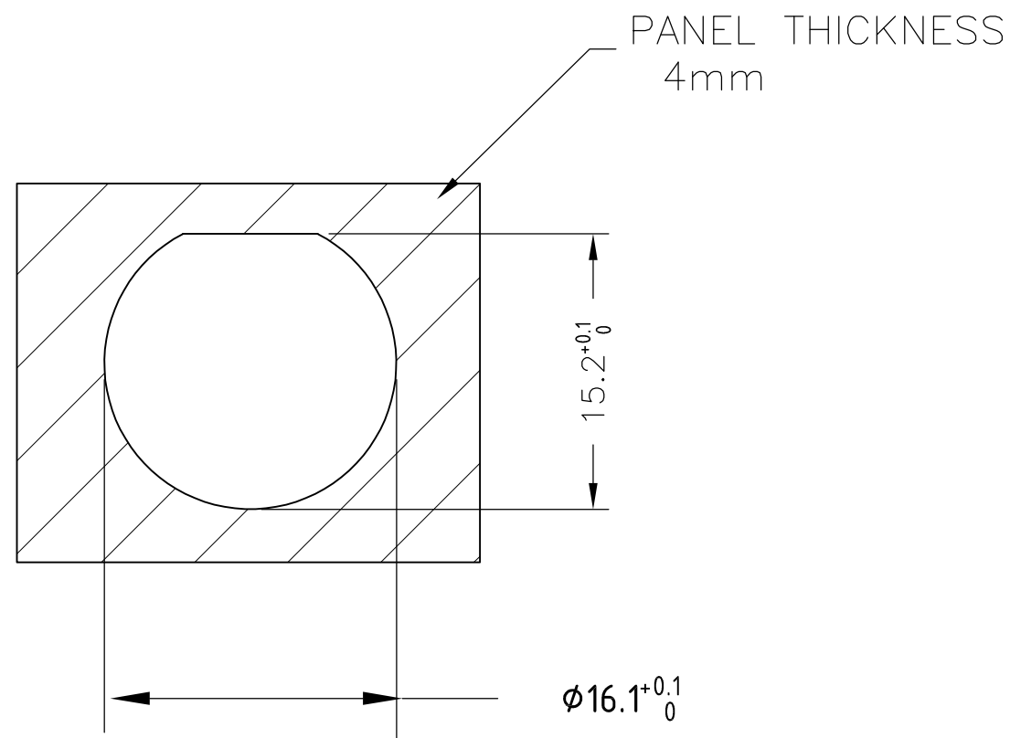
PANEL CUTOUT
