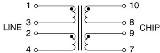
SCHEMATIC
