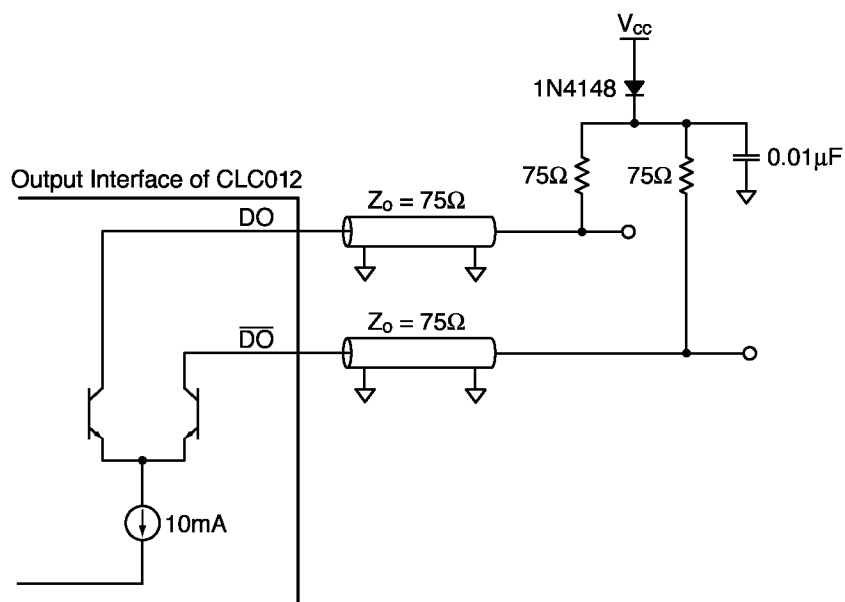
Figure 6. Differential Load Terminated Output Interface
