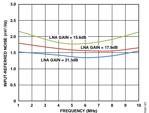
Figure 14. Short-Circuit, Input-Referred Noise vs. Frequency, PGA \text{ Gain} = 30 \text{ dB} , GAIN+ = 1.6 V
