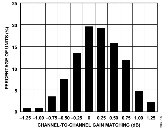
Figure 10. Gain Match Histogram, GAIN+ = 0.3 V
