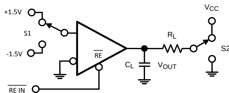
Figure 16. Test Circuit for Receiver Enable / Disable
