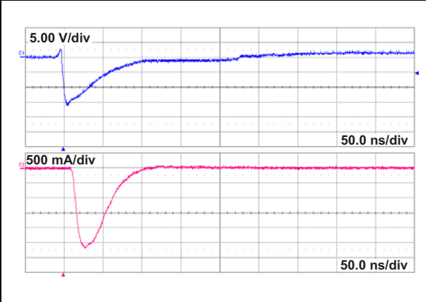
Figure 8. Response to ISO 7637-3 (pulse 3a) U_S = -150\text{ V}
