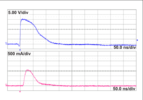
Figure 9. Response to ISO 7637-3 (pulse 3b) U_S = 100\text{ V}
