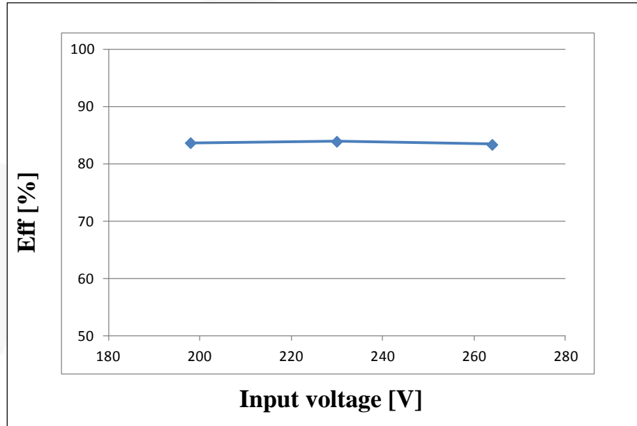
Figure 18. System Efficiency
