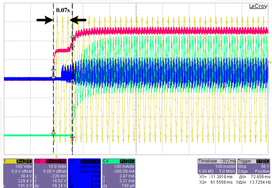
Figure 9. V_{IN} = 230\text{ V}_{AC} / 50\text{ Hz}
