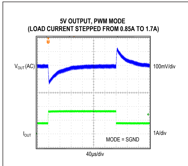
Figure 10. MAX17545 5V Output, 0.85A to 1.7A Load Transient
