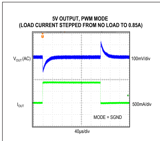
Figure 7. MAX17545 5V Output, No Load to 0.85A Load Transient (PWM Mode)
