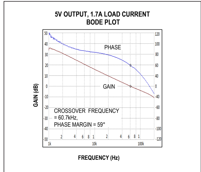
Figure 6. MAX17545 5V Output Full Load Bode Plot ( V_{IN} = 24V )
