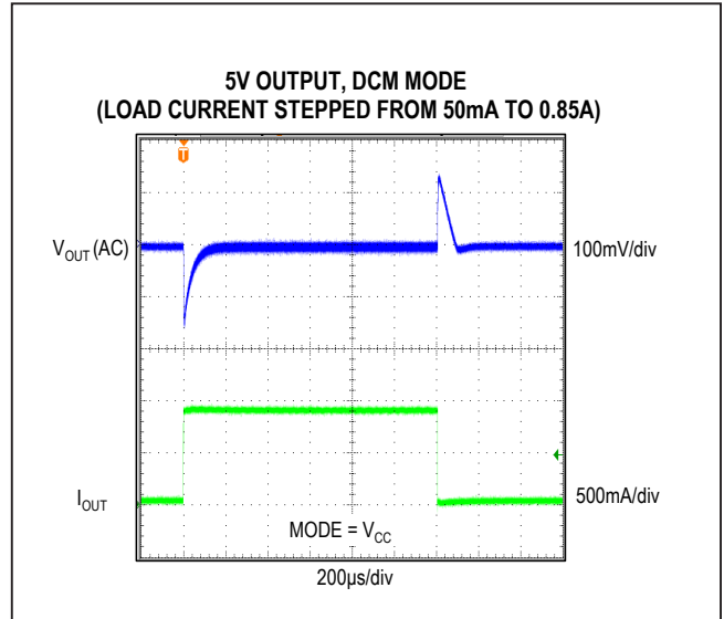
Figure 9. MAX17545 5V Output, 50mA to 0.85A Load Transient (DCM Mode)
