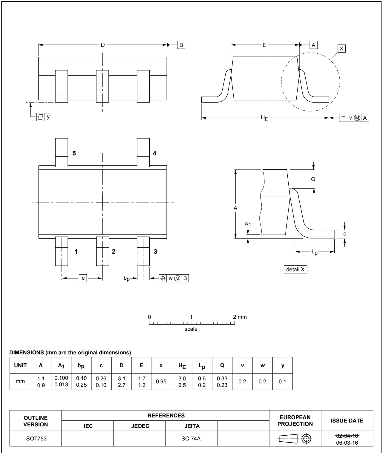
Figure 12. Package outline SOT753
