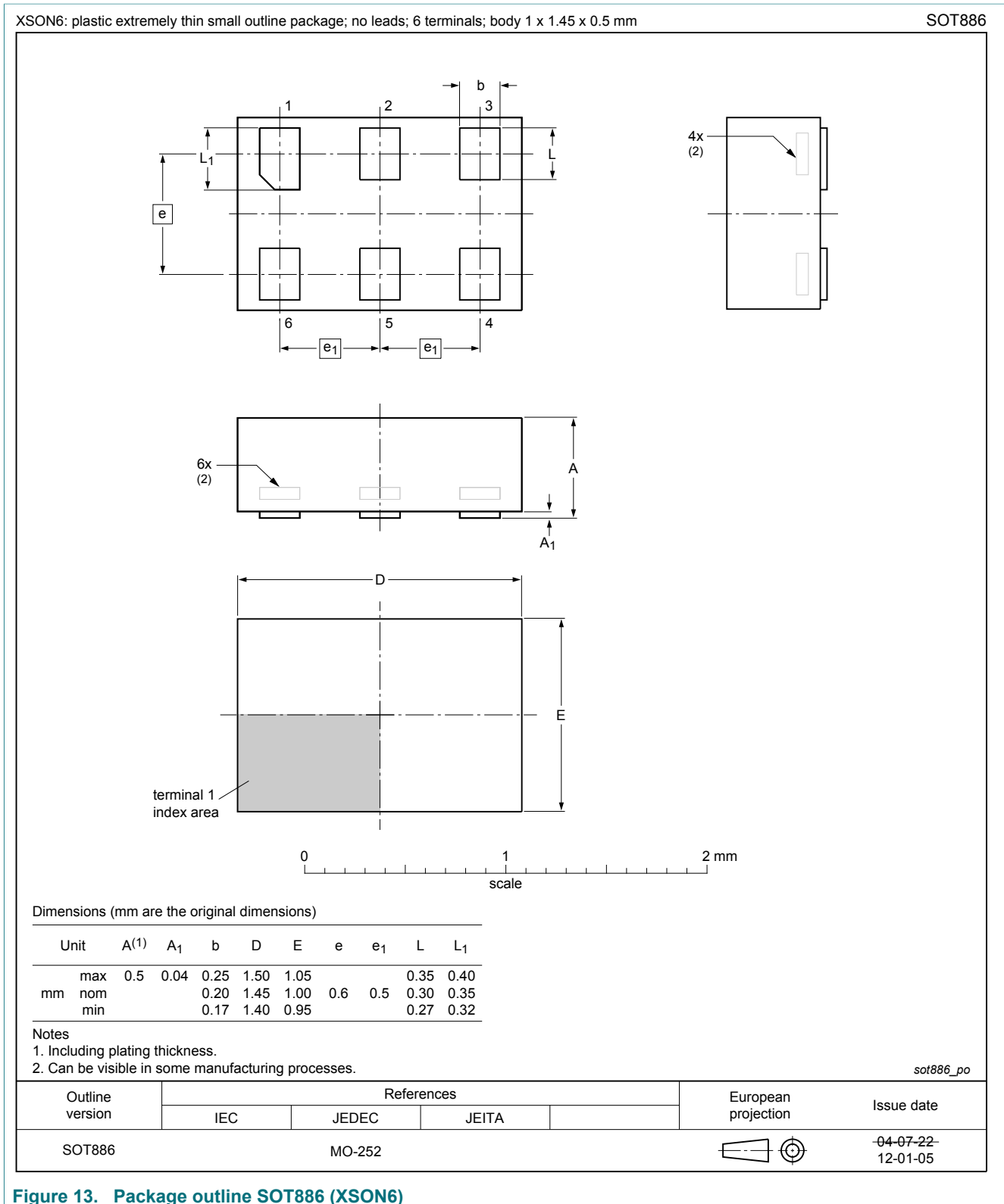
Figure 13. Package outline SOT886 (XSON6)
