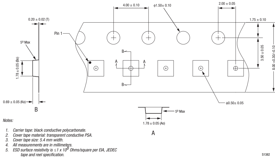
Figure 8. SKY13523-639LF Tape and Reel Dimensions
