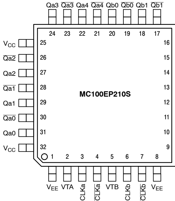
Figure 1. 32-Lead LQFP Pinout (Top View)
