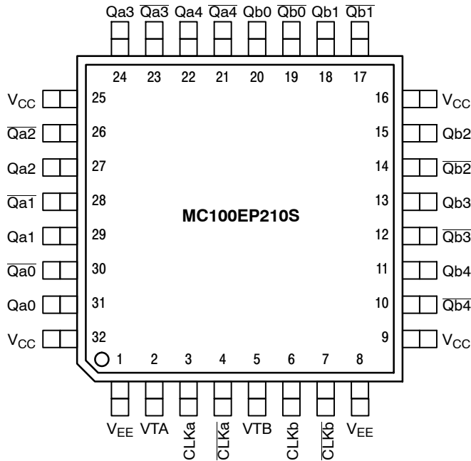
Figure 1. 32-Lead LQFP Pinout (Top View)
