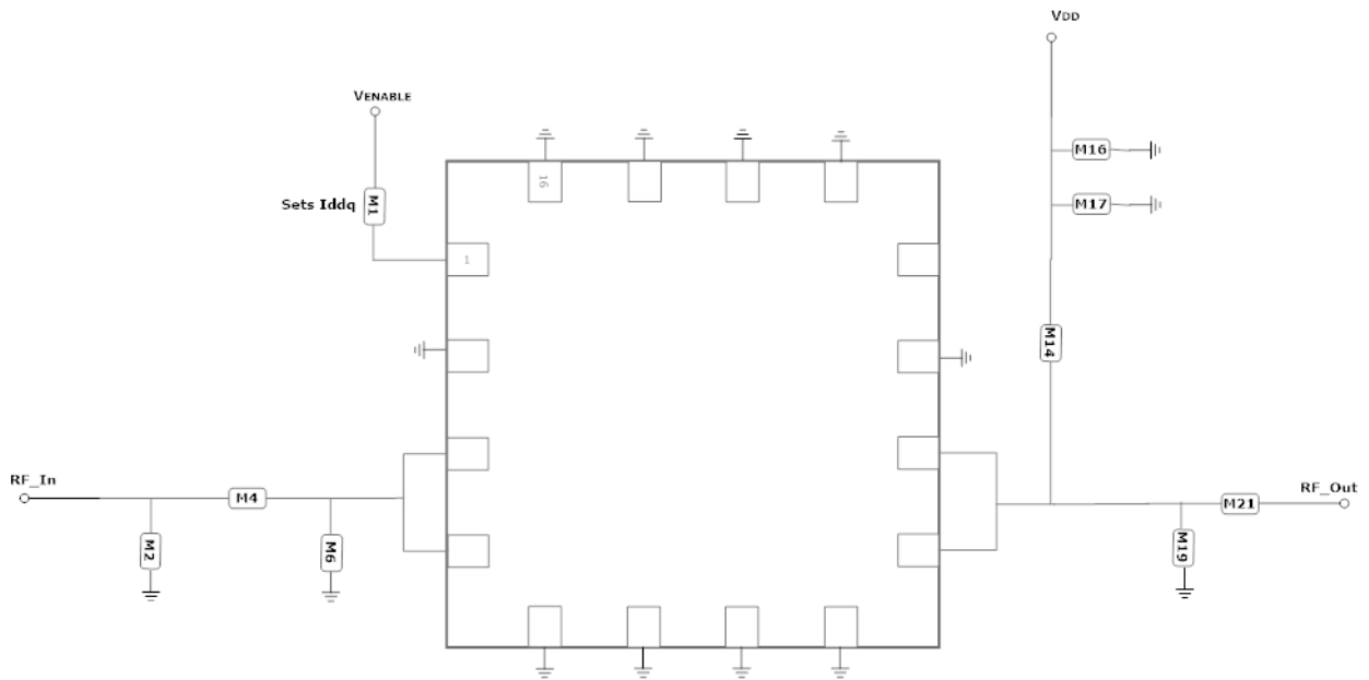
GRF5020 Application Schematic: (1.7 to 2.7 GHz)
