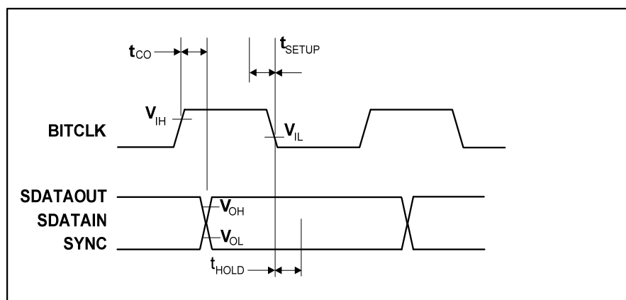
Figure 18 Data Setup and Hold (50pF External Load)
