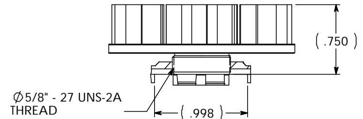
DETAIL A SCALE = 6X
