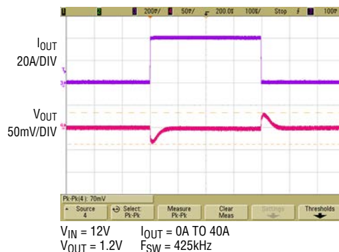
Figure 5. Load Transient Waveform DC1740A-A
