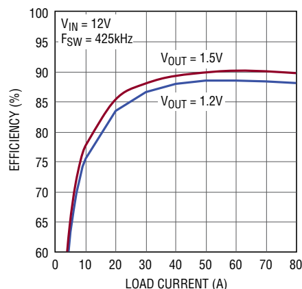
Figure 4. Typical Efficiency Curves DC1740A-A
