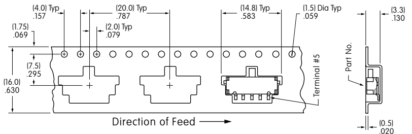
Tape Dimensions
