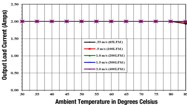
UWS-24/2-Q12N-C Temperature Derating Vin 24V (air flow from Pin 1 to Pin 3 on PCB)
