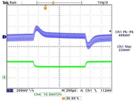
Step Load Transient Response ( V_{in}=24V , V_{out}=\text{nom.} , I_{out}=50\text{-}75\text{-}50\% of full load, C_{load}=1\mu\text{F} ceramic II 10\mu\text{F} tantalum, T_a=+25^\circ\text{C} , ScopeBW=20MHz)
