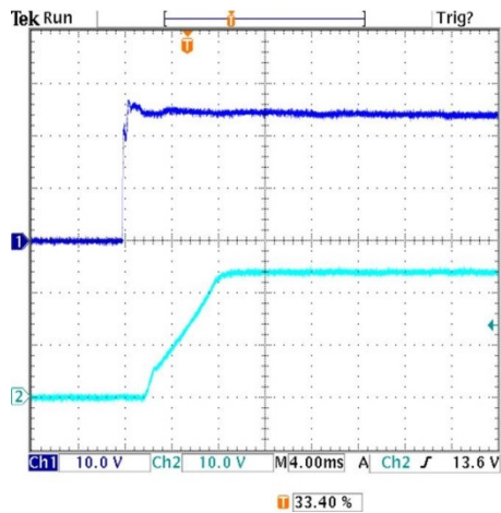
Power On Startup Delay ( V_{in}=0 to 24V , V_{out}=\text{nom.} , I_{out}=\text{no load} , C_{load}=0\mu\text{F} , T_a=+25^\circ\text{C} , ScopeBW=20MHz) Trace 1= V_{in} , Trace 2= V_{out}
