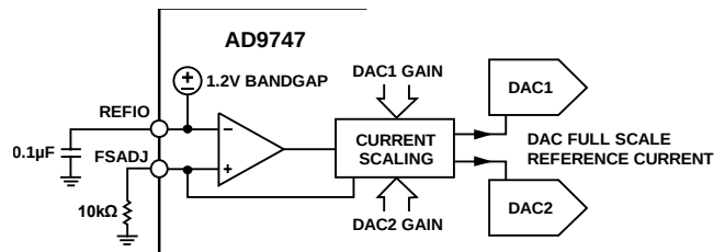
Figure 33. Reference Circuitry
