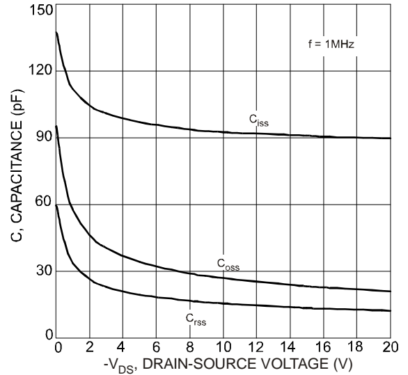
Fig. 10 Typical Capacitance
