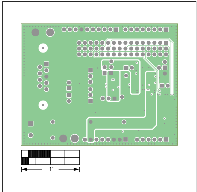
MAX13053A Shield—Internal 3
