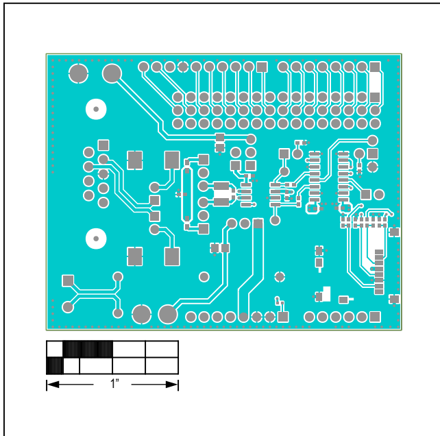
MAX13053A Shield—Top
