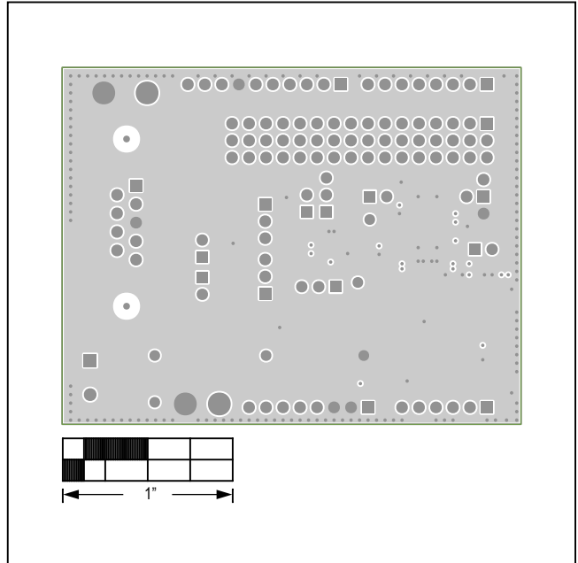
MAX13053A Shield—Internal 2
