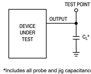
Figure 2. Test Circuit
